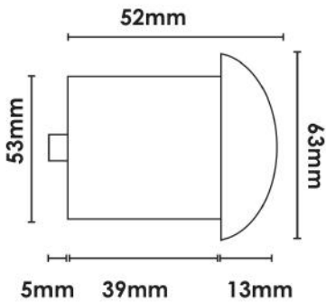
CUTOUT WITHOUT CANISTER Ø54mm
