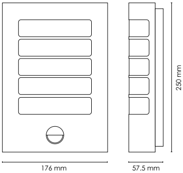
Model: Stark LED Wall Light with Sensor
