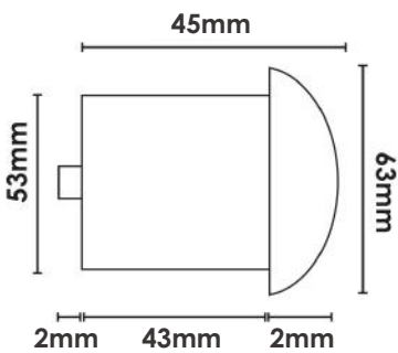
CUTOUT WITHOUT CANISTER Ø54mm
