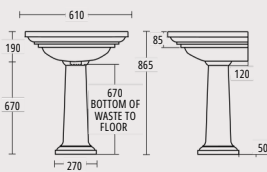
Medium basin and pedestal
