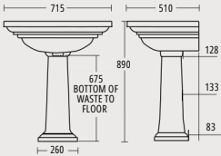
Large basin and pedestal
