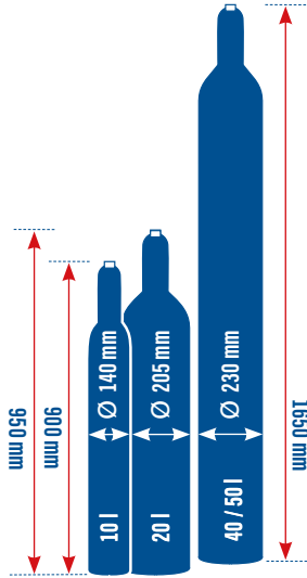
1 Gas cylinder
