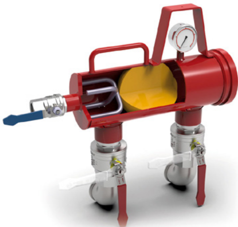
Premier Pipeline's new-style blow-out cannon
