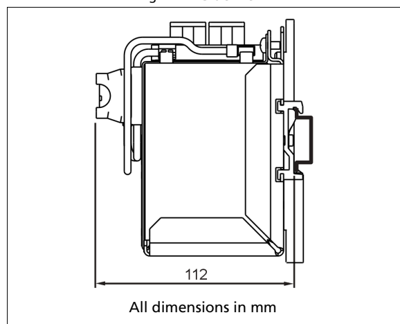
Fig. 12-2 Side view
