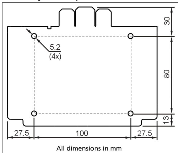
Fig. 13-2 Hole pattern for wall mount
