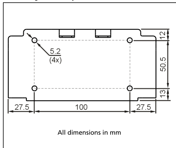
Fig. 13-3 Hole pattern for bottom mount
