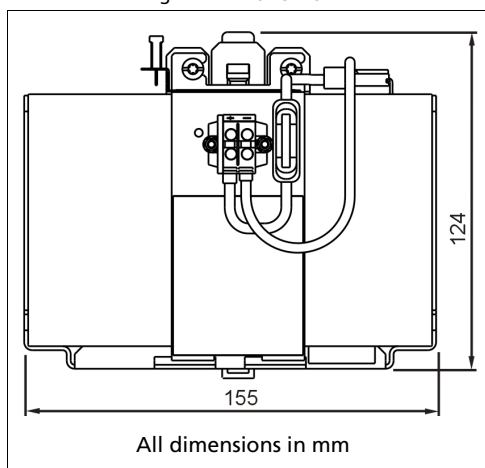
Fig. 12-1 Front view
