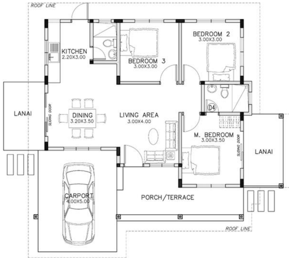
FLOOR PLAN
