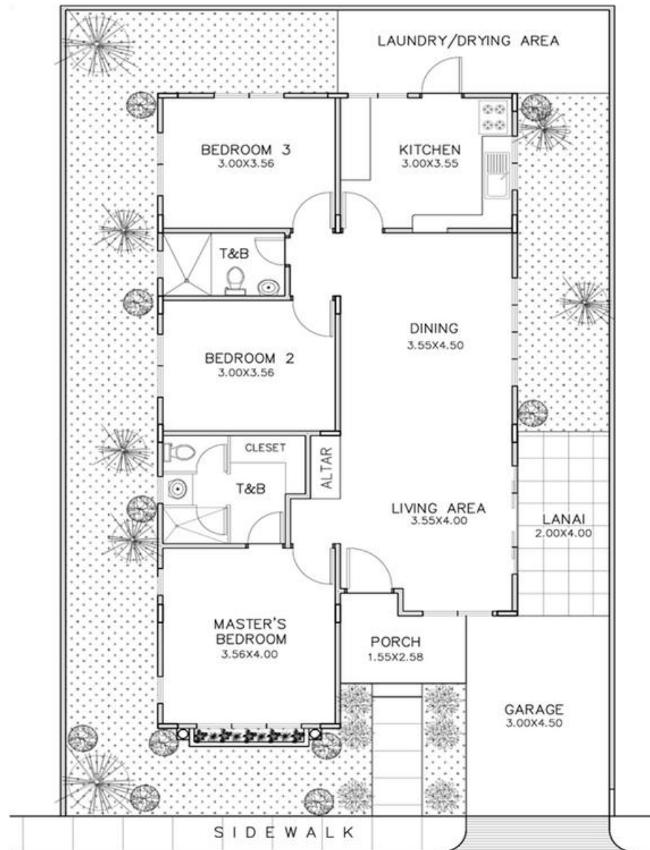
FLOOR PLAN
