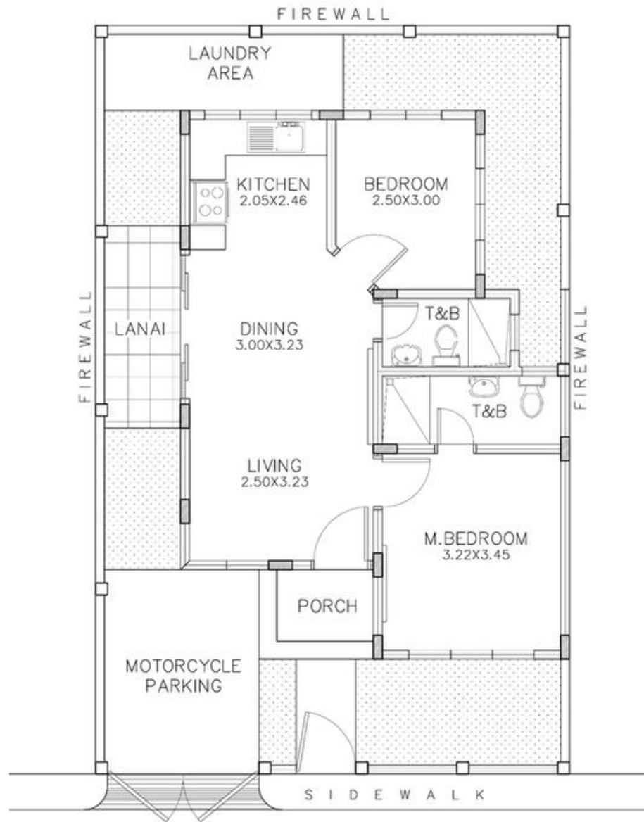
FLOOR PLAN
