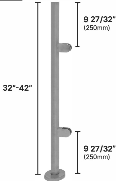
End Post
