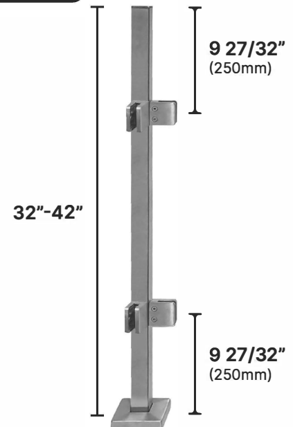
Corner Post
