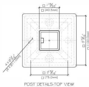
POST DETAILS-TOP VIEW
