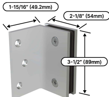
WMB90 Square Wall Mount Bracket - 90°
