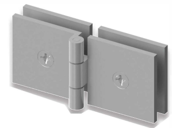
SQCADJ188 * Square Adjustable Glass to Glass Clamp with Hinge
