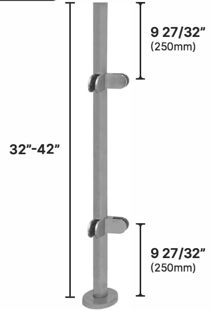
Corner Post
