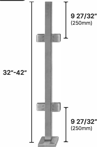
Inline Post
