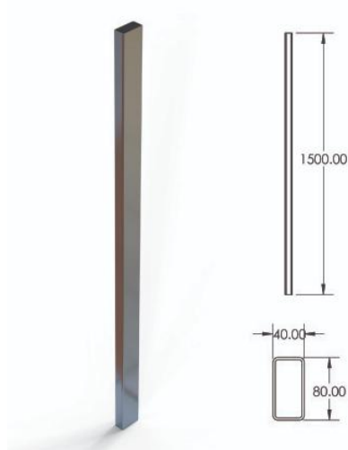
1.5M BOX STEEL GROUND FIXING
