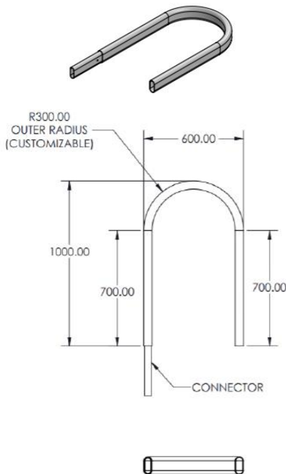
BULLNOSE
