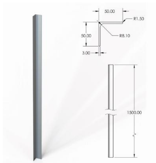
1.5M STEEL ANGLE
