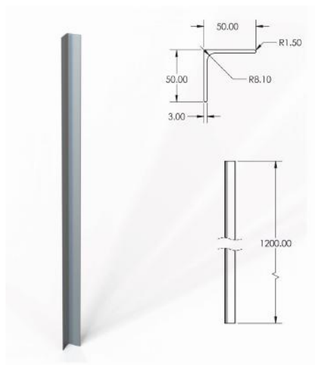
1.2M-STEEL ANGLE
