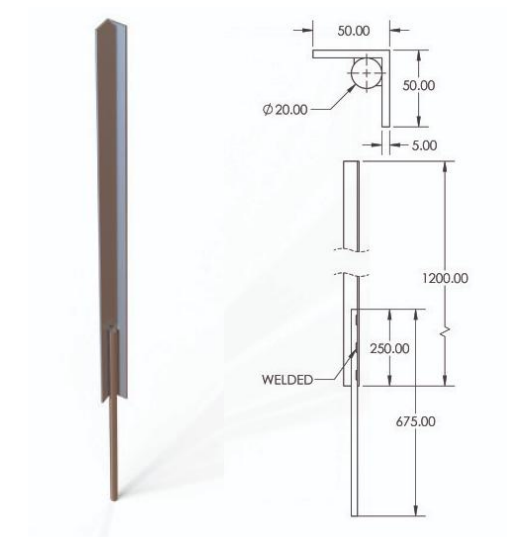
PUTLOCK-1200
