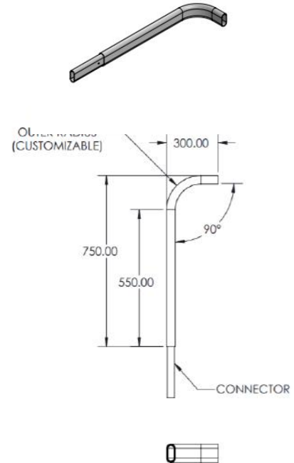
FAIRING END
