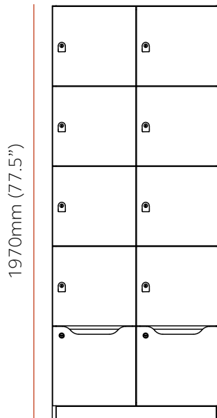
8 door, 2 drawers
