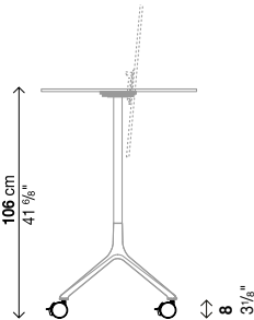
Kit ruote/castors
