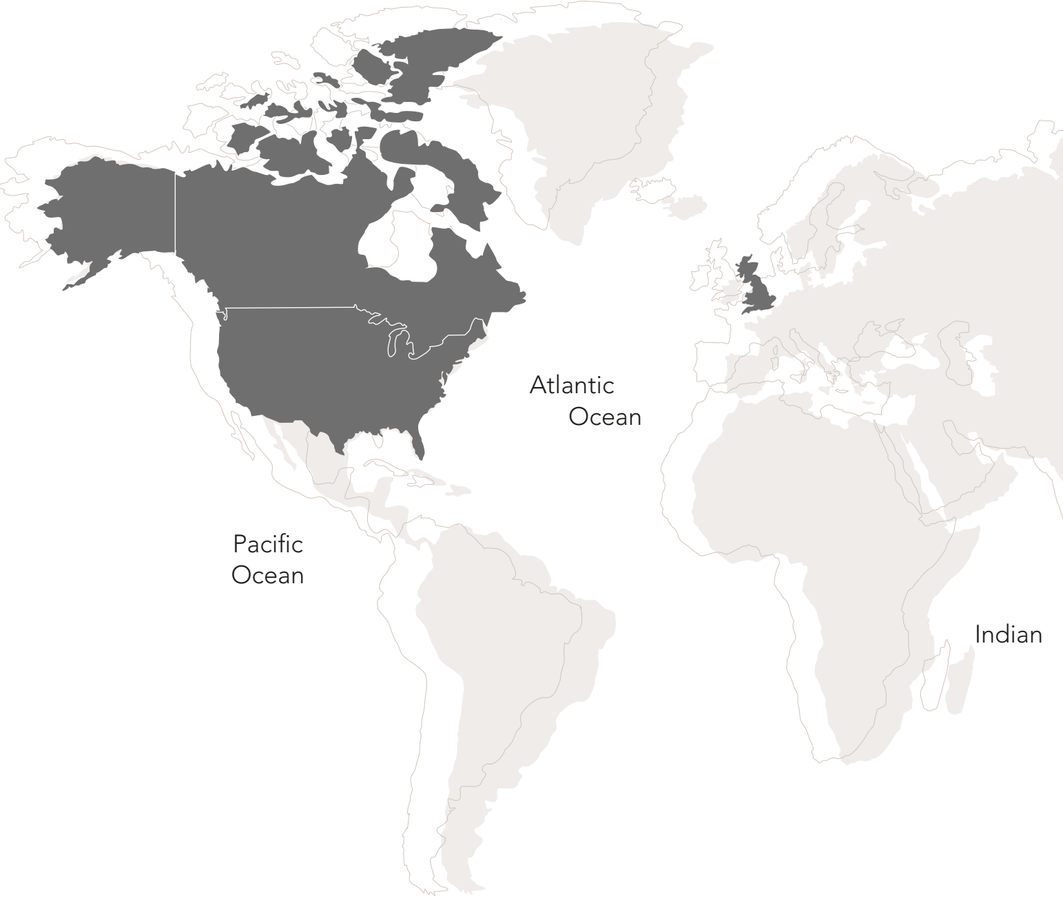
WHITE TOULIPIER
