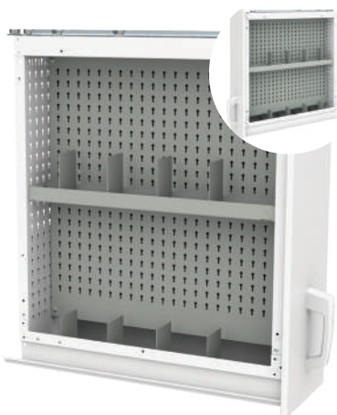
Adjustable utility panel 1 , 2 trays, 16 magnetic dividers 3
