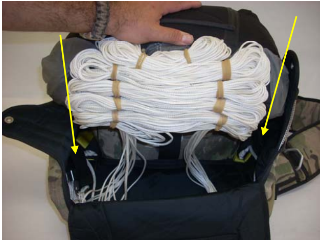
Tuck the Risers along the Reserve tray.
