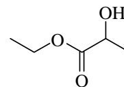
2. Ethyl lactate
