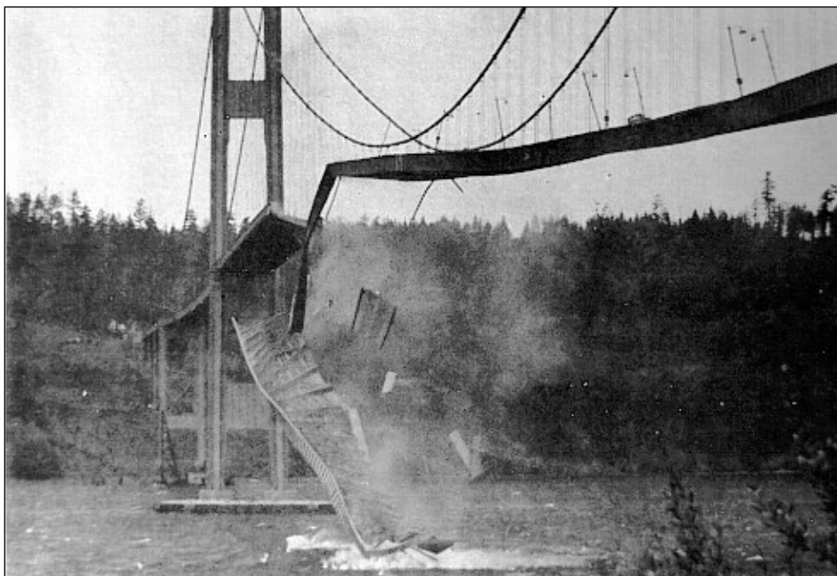
Figure 4.5-6 Tacoma Narrows Bridge – November 7, 1940, Windstorm
