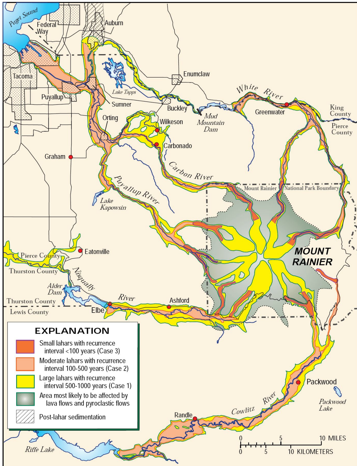
Map 4.7-1 Lahars, Lava Flows, and Pyroclastic Hazards of Mt. Rainier 6
