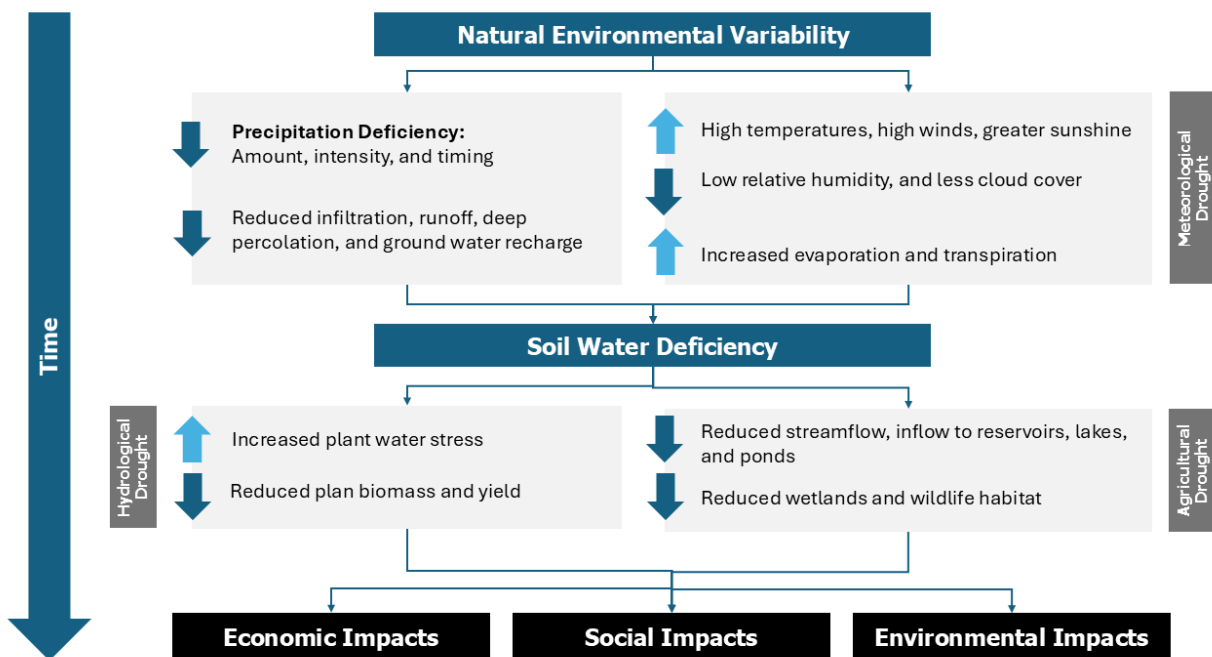
Figure 4.1-1 Sequence of Drought Impacts 3
