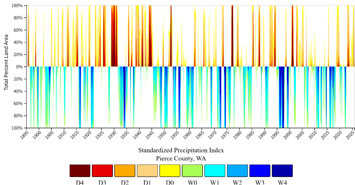
Figure 4.1-3 Historical Standardized Precipitation Index in Pierce County, 1895 to 2025
