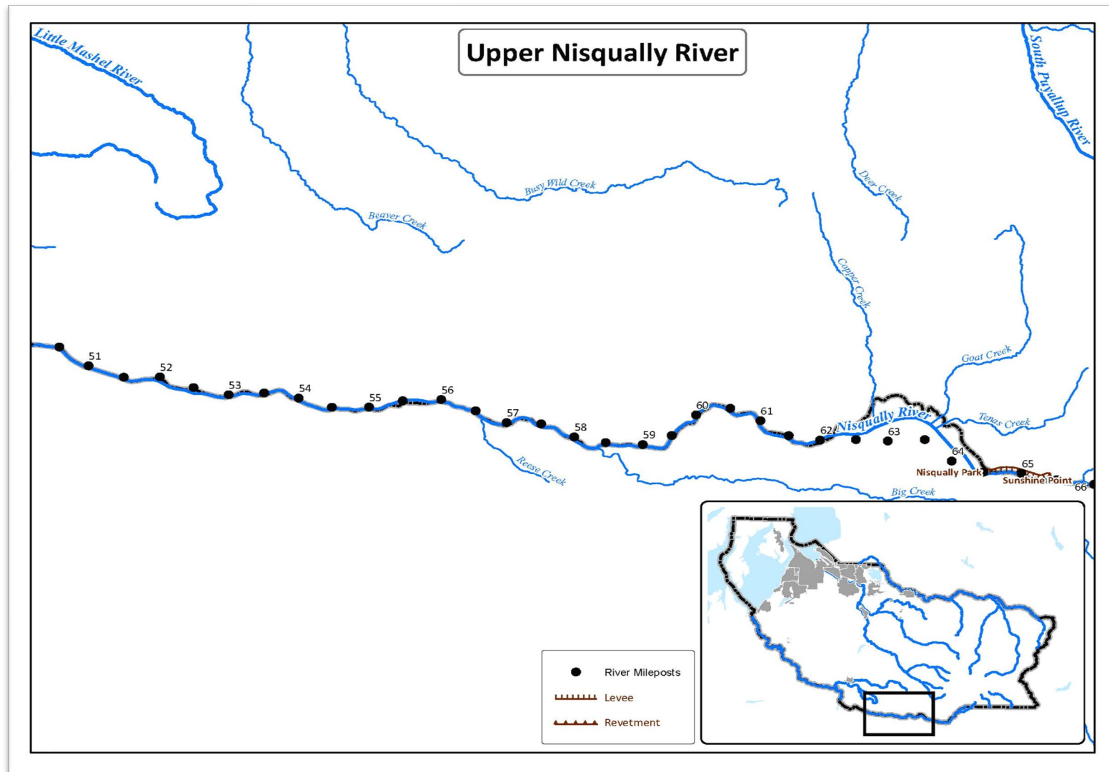
Map 4.3-11 Upper Nisqually River
