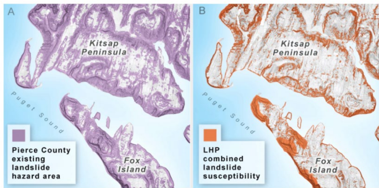
Figure 4.4-3 Pierce County Comparison of Landslide Susceptible Areas
