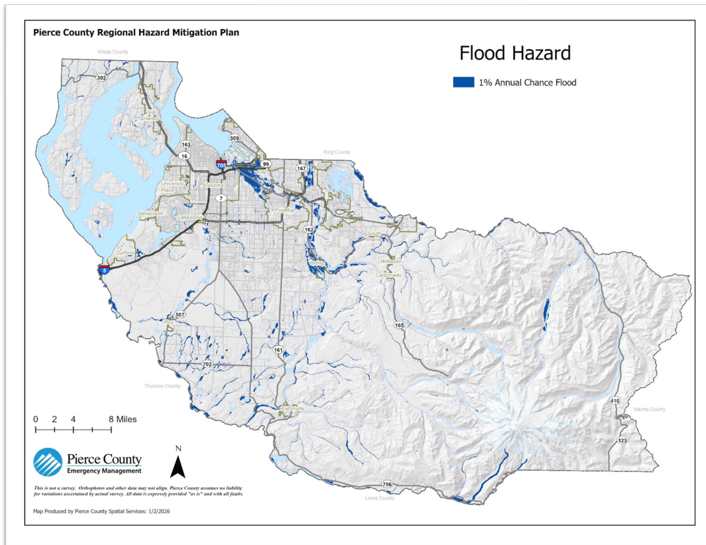
Map 4.3-1 Map Showing Mapped 1% Annual Chance Floodplains and Floodways in Unincorporated Pierce County
