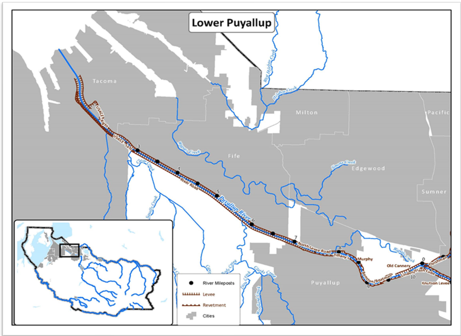
Map 4.3-2 Lower Puyallup River
