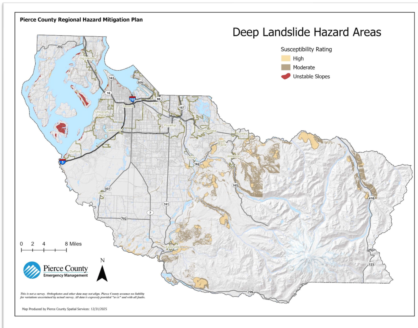
Map 4.4-1 Pierce County Deep Landslide Hazard Area
