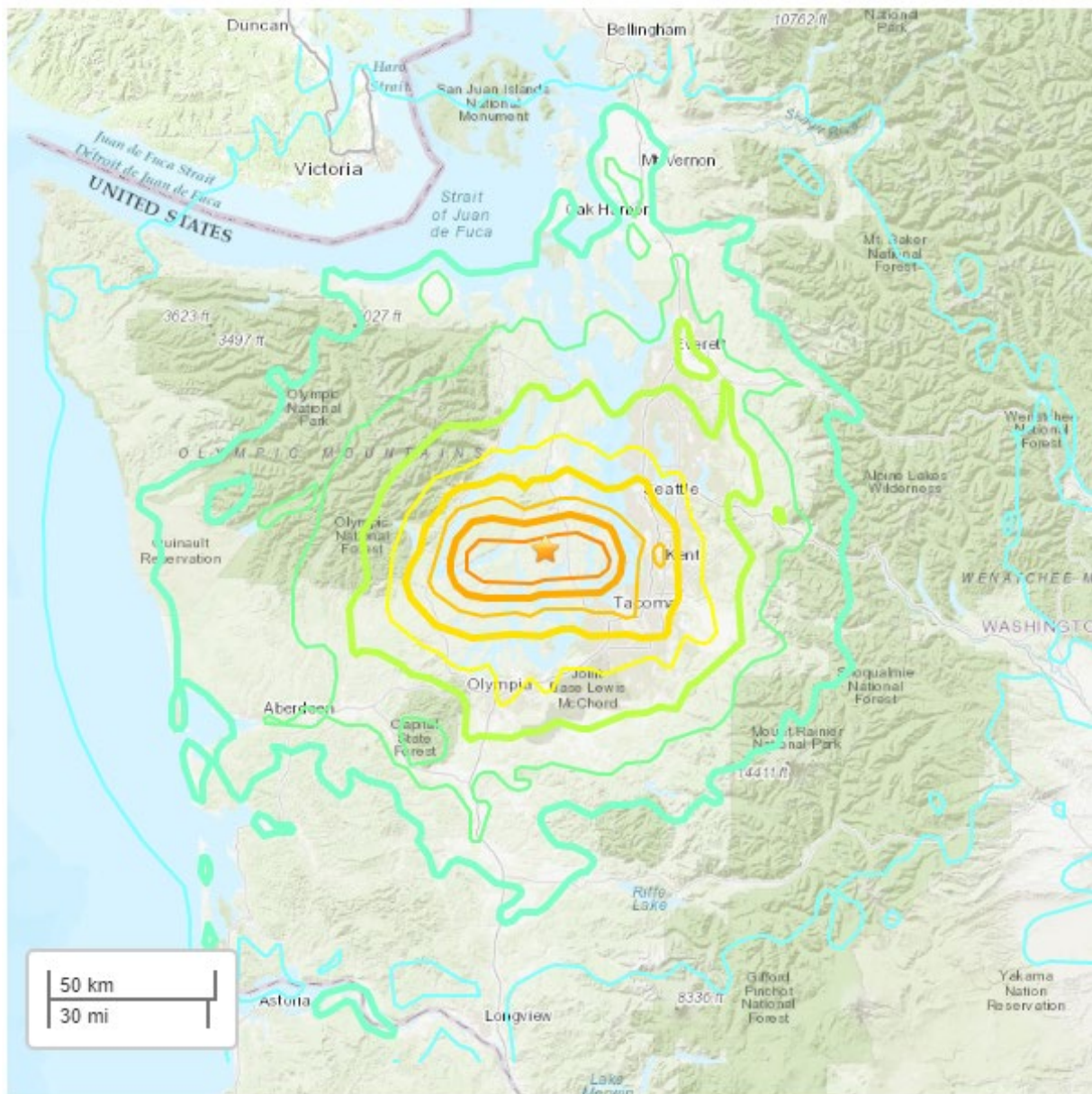
Figure 4.2-4 Magnitude 6.9 Scenario Earthquake – Tacoma Fault Zone 9.0 km depth
