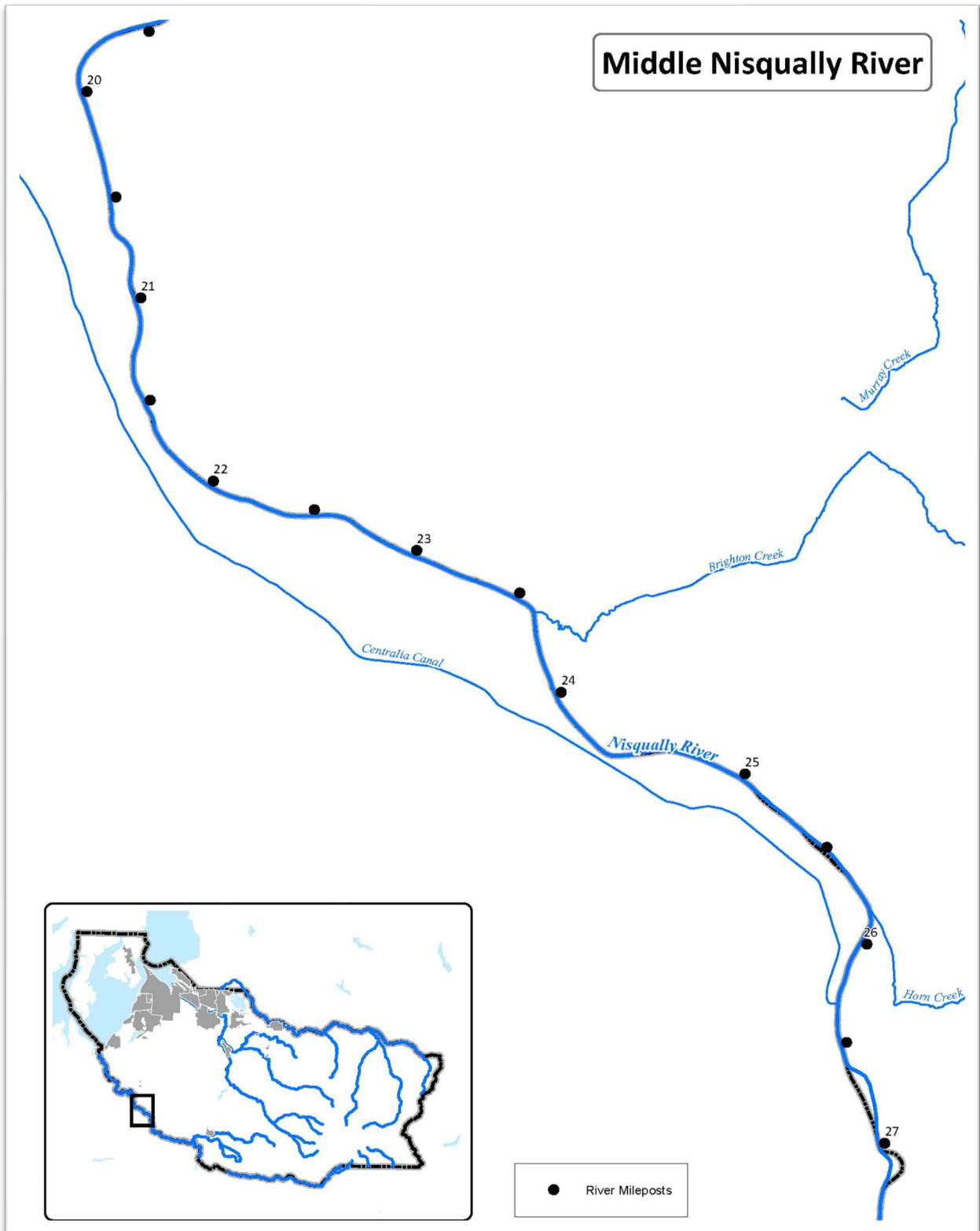
Map 4.3-10 Middle Nisqually River
