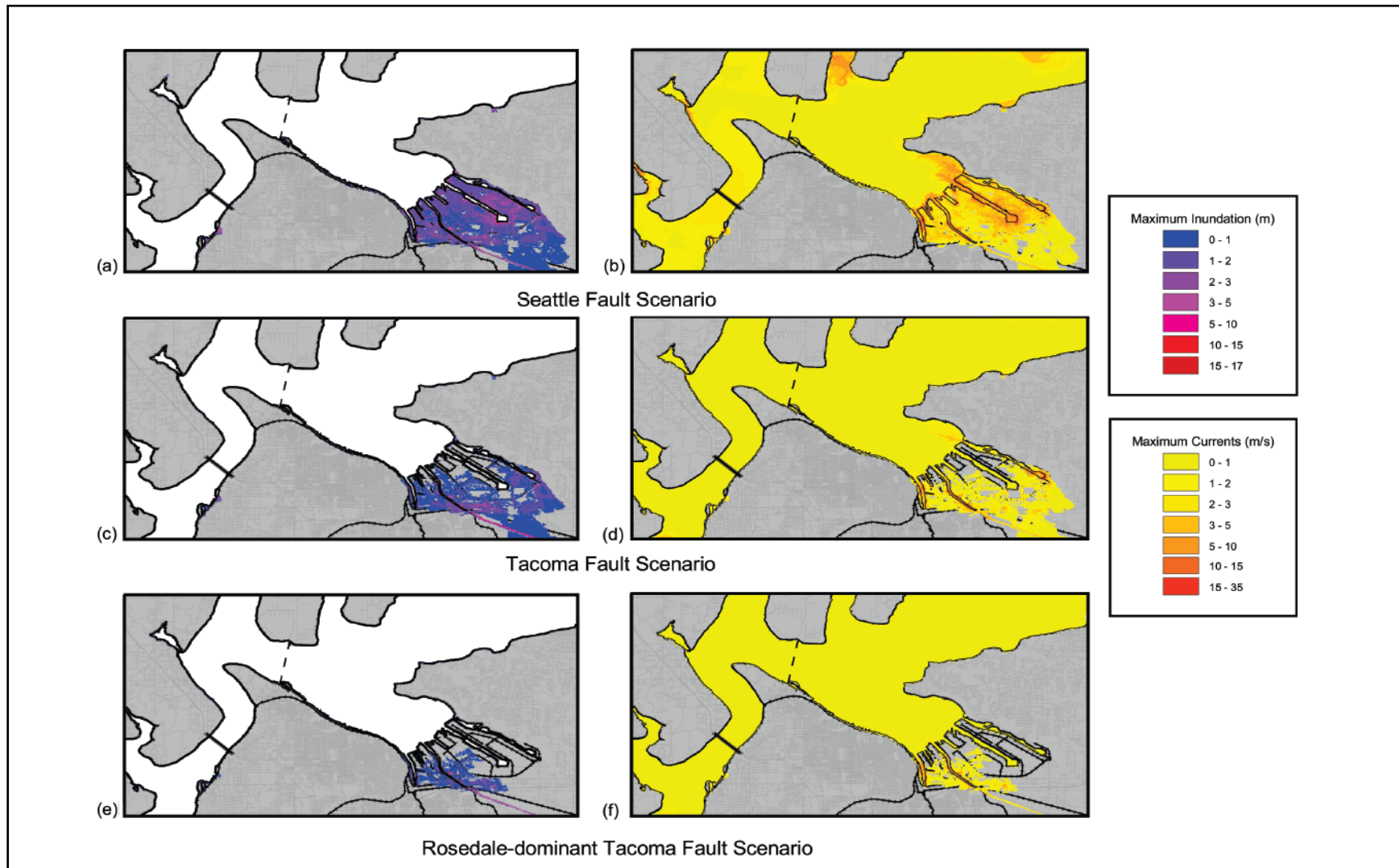
Figure 4.6-4 Tsunami Inundation and Current-Based on Earthquake Scenario 7
