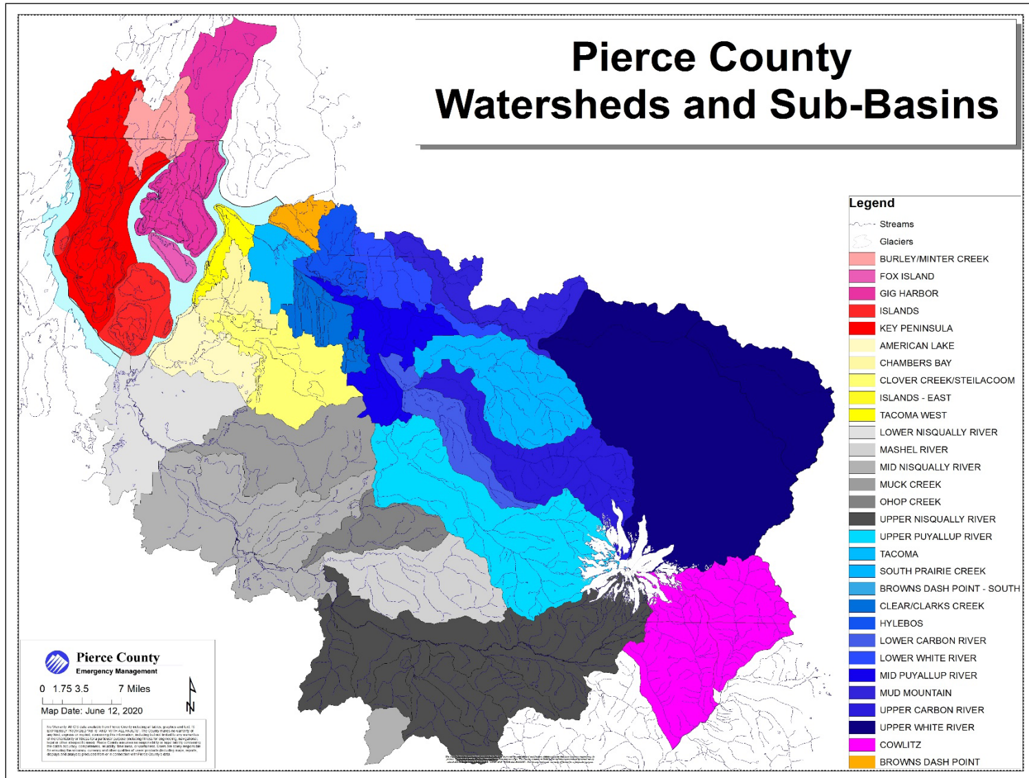
Map 4.1-1 Pierce County Watersheds
