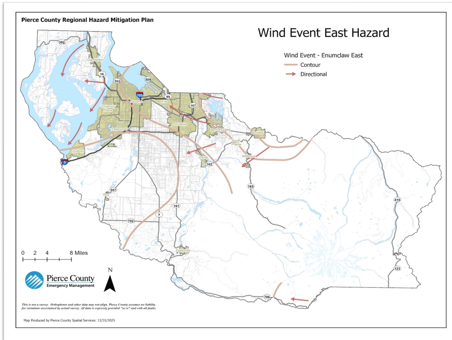
Map 4.5-2 Pierce County Severe Weather Wind Hazard – East-Wind Event
