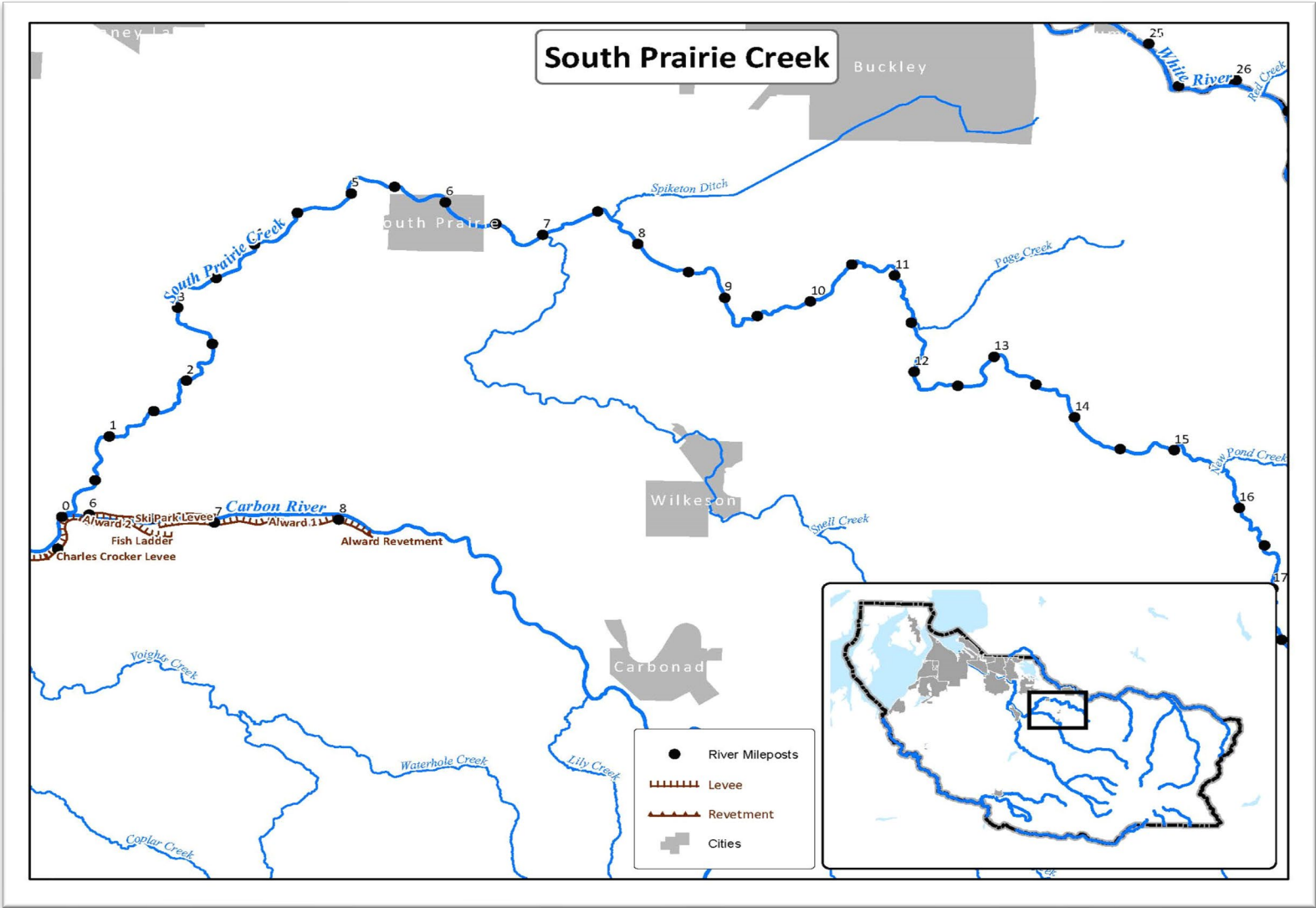
Map 4.3-9 South Prairie Creek
