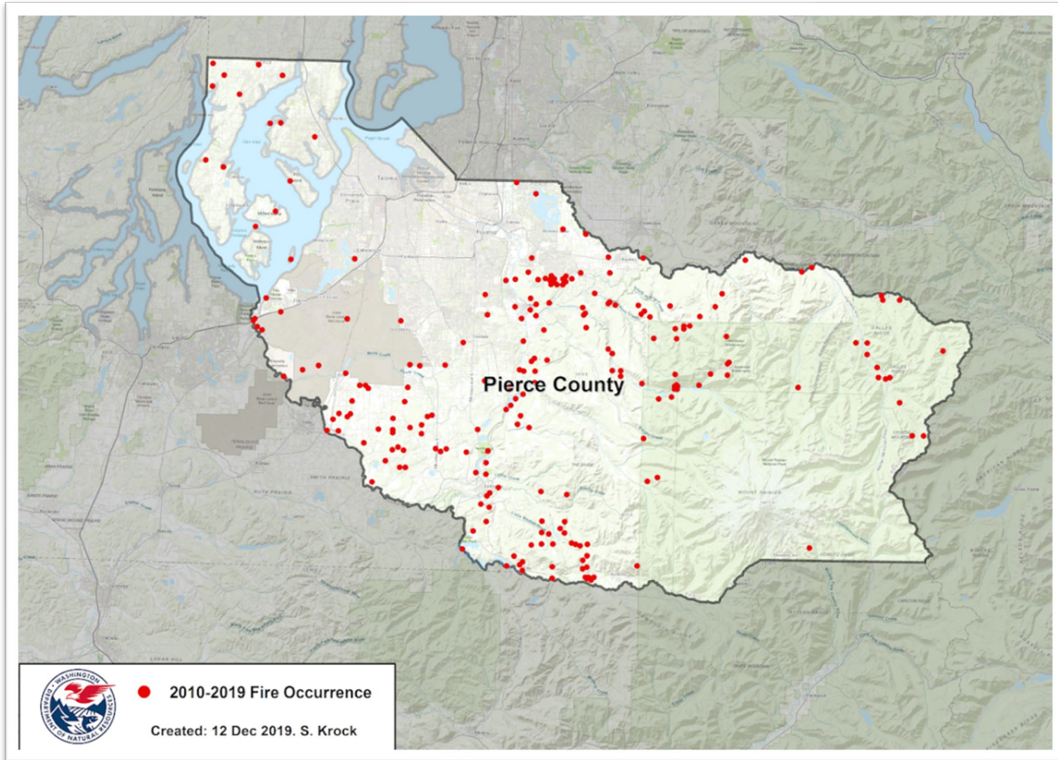
Map 4.8-3 Pierce County Fire Occurrences from 2010 to 2019
