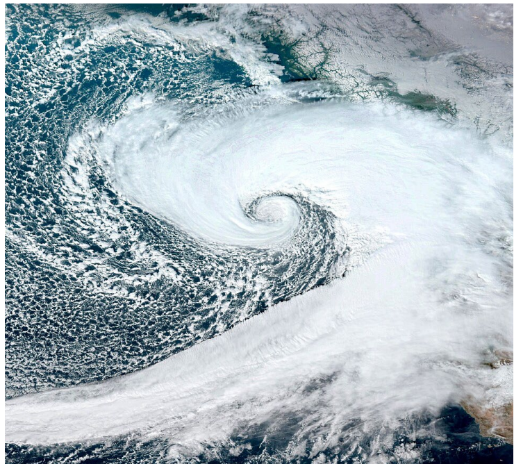
Figure 4.5-2 Satellite image of the November 2024 Northeast Pacific bomb cyclone, as seen on 19 November 2024. 6
