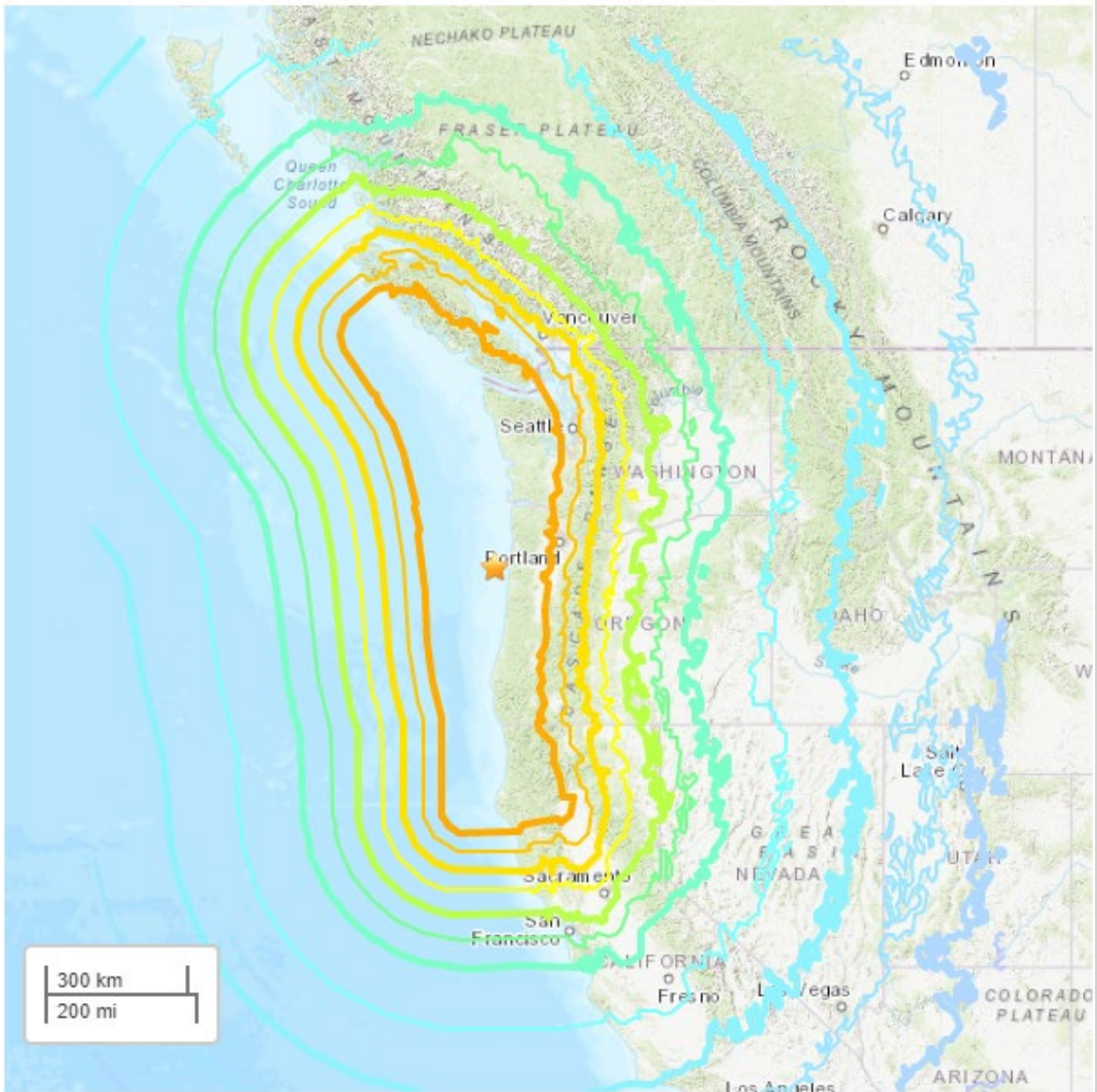
Figure 4.2-6 Magnitude 9.3 Scenario Earthquake – Cascadia Megathrust – 21.4km depth
