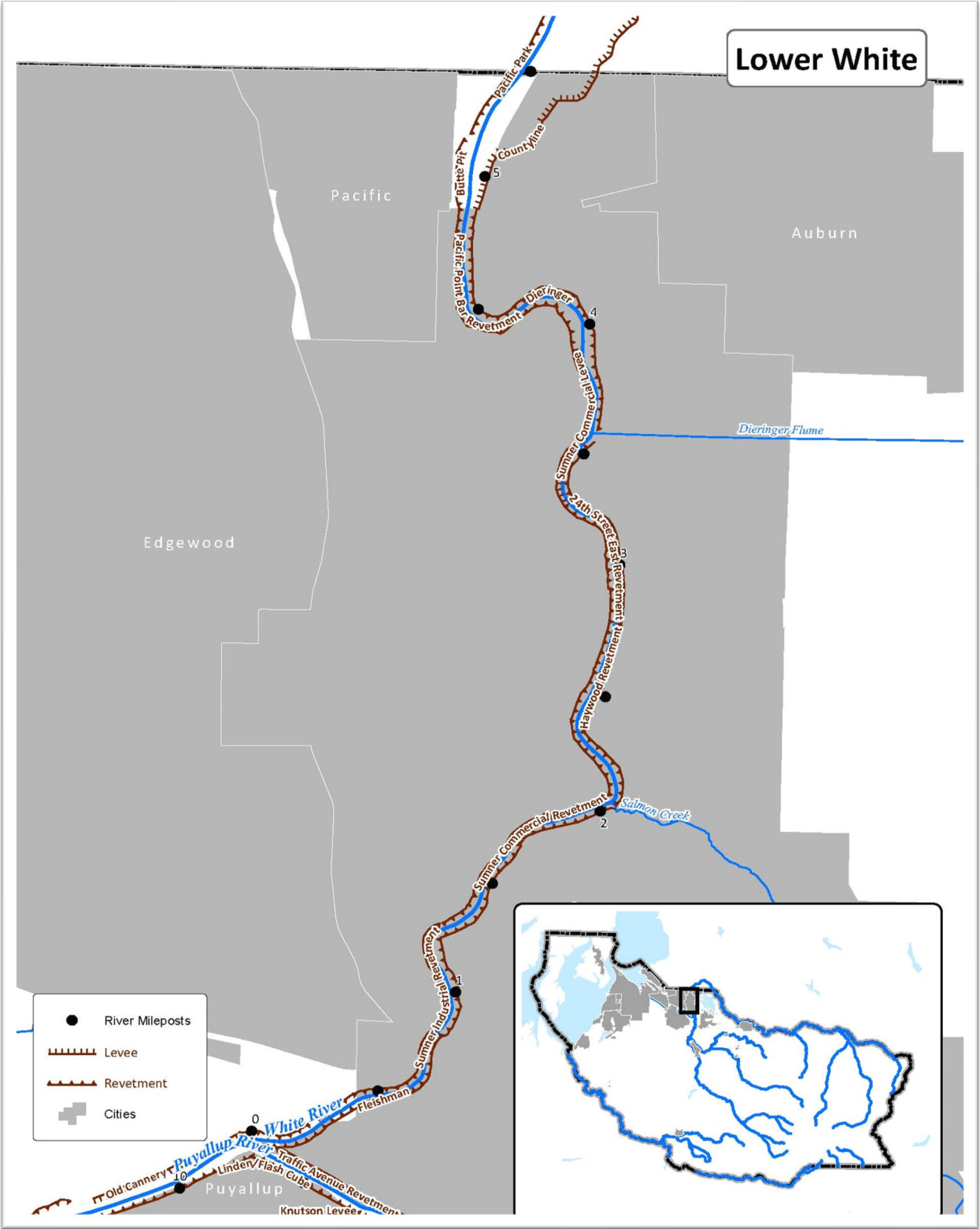
Map 4.3-5 Lower White River
