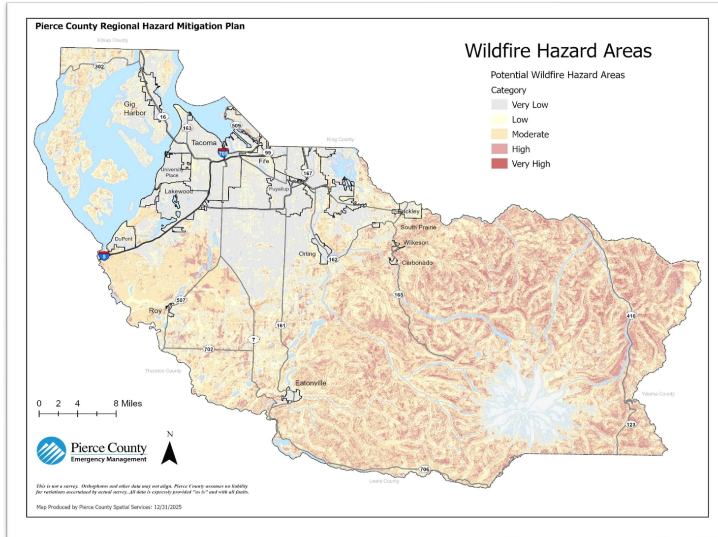
Map 4.8-1 Wildfire Hazard Areas
