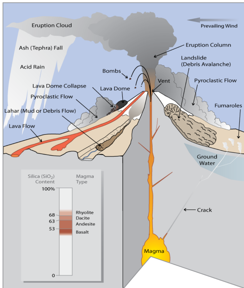
Figure 4.7-1 Volcanic Hazards 1
