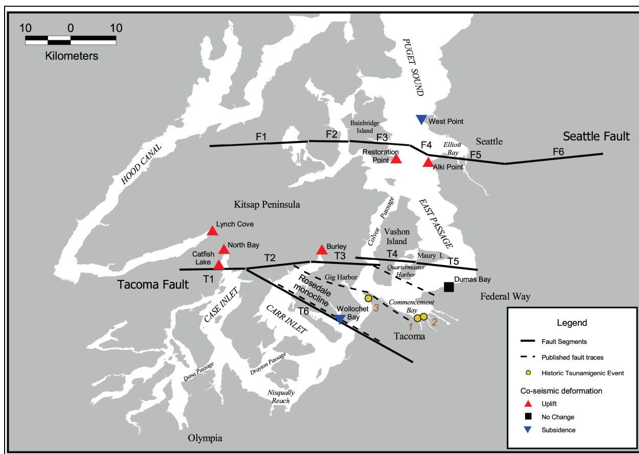
Figure 4.6-3 Seattle and Tacoma Faults 5
