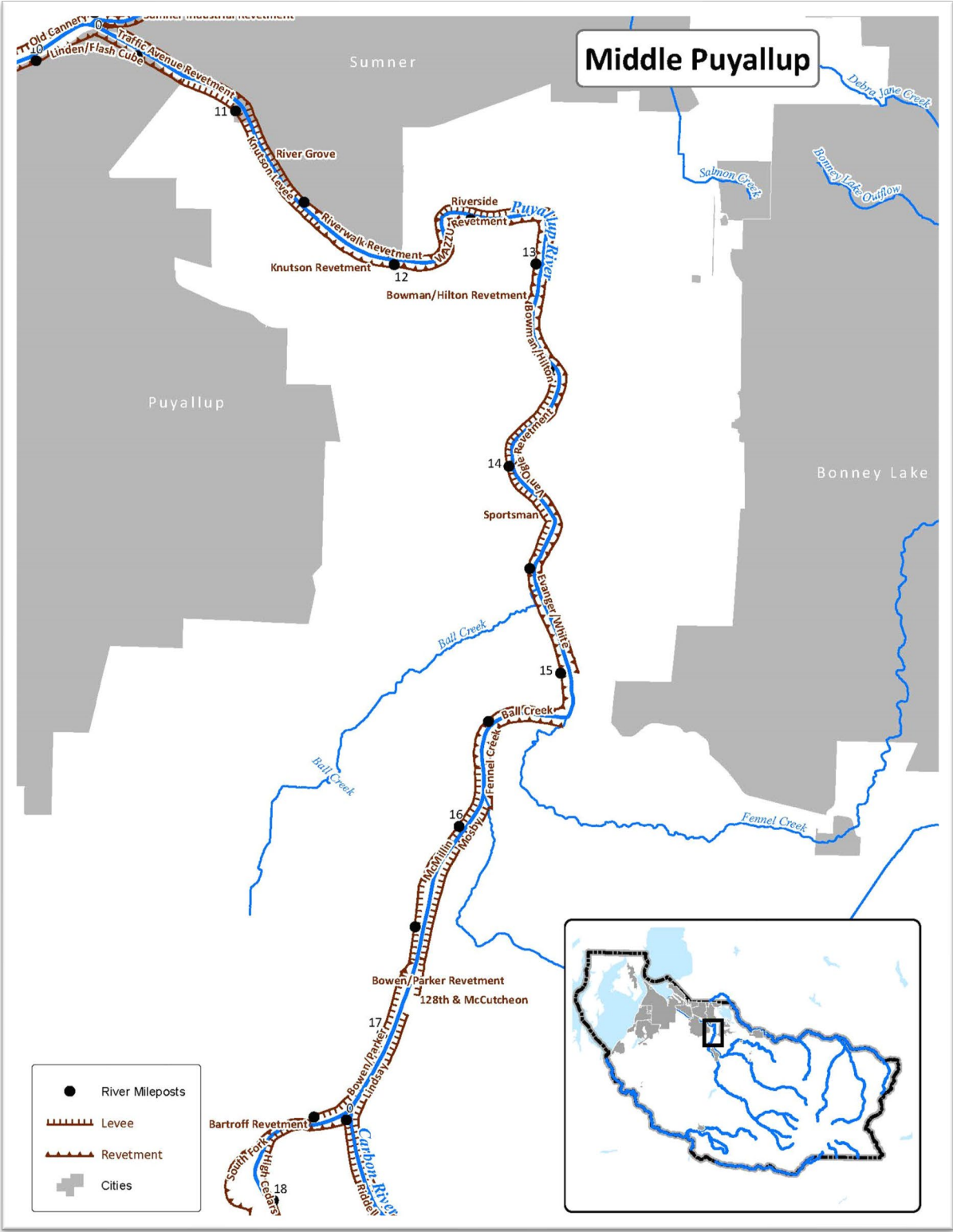
Map 4.3-3 Middle Puyallup River
