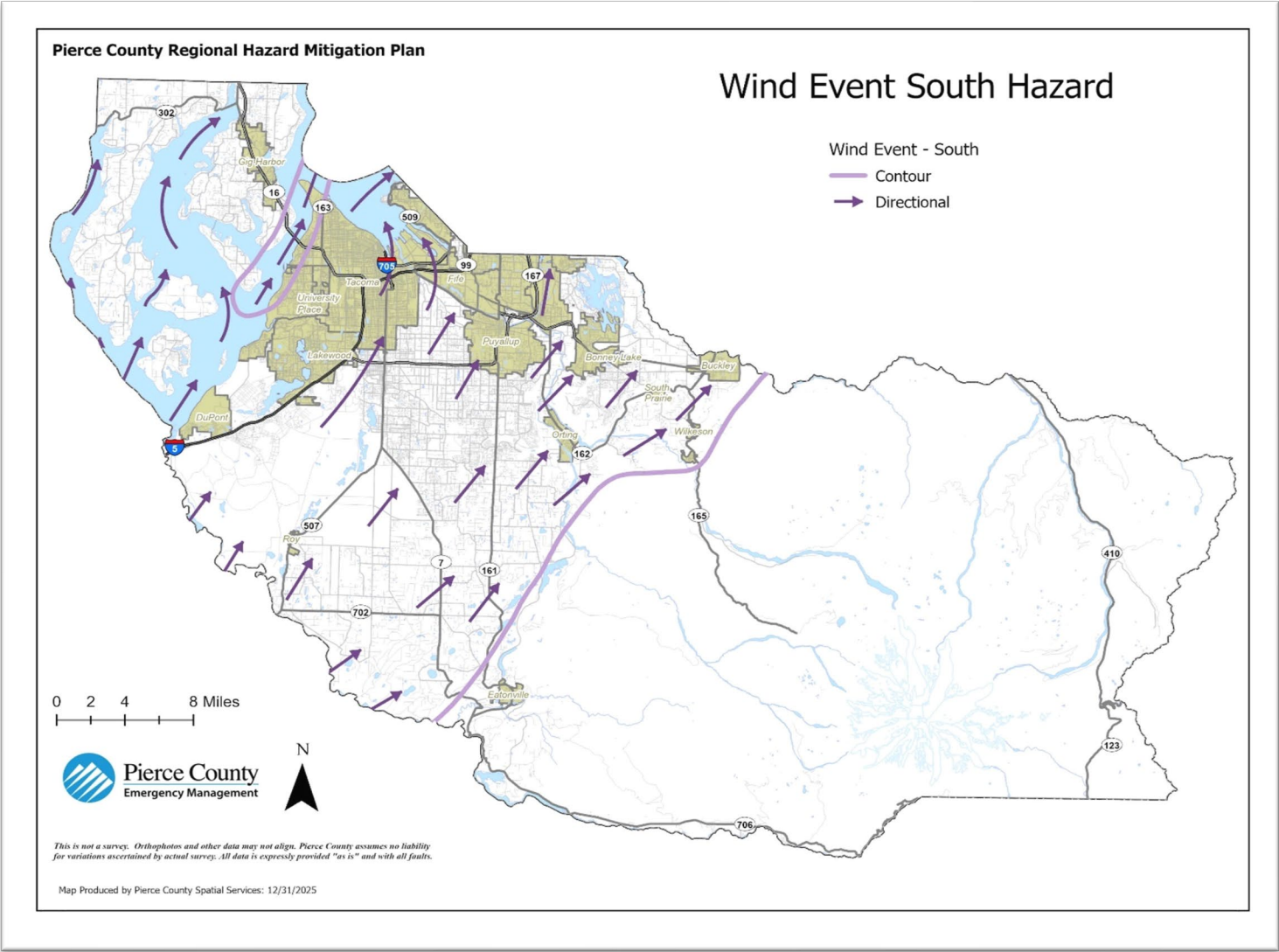
Map 4.5-1 Pierce County Severe Weather Wind Hazard – South-Wind Event
