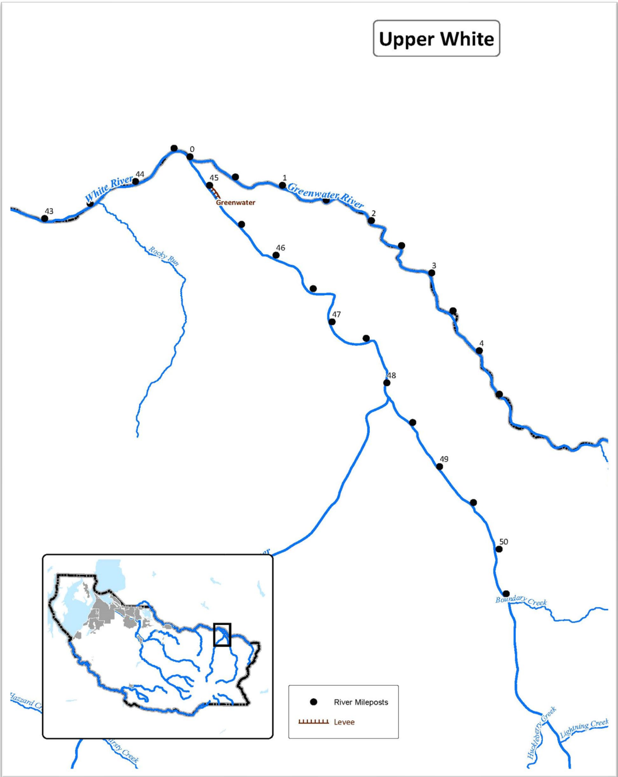
Map 4.3-6 Upper White River
