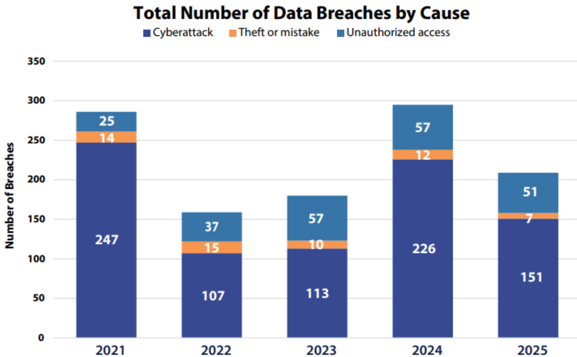
Figure 4.2-1 Total Number of Data Breaches by Cause in Washington State
