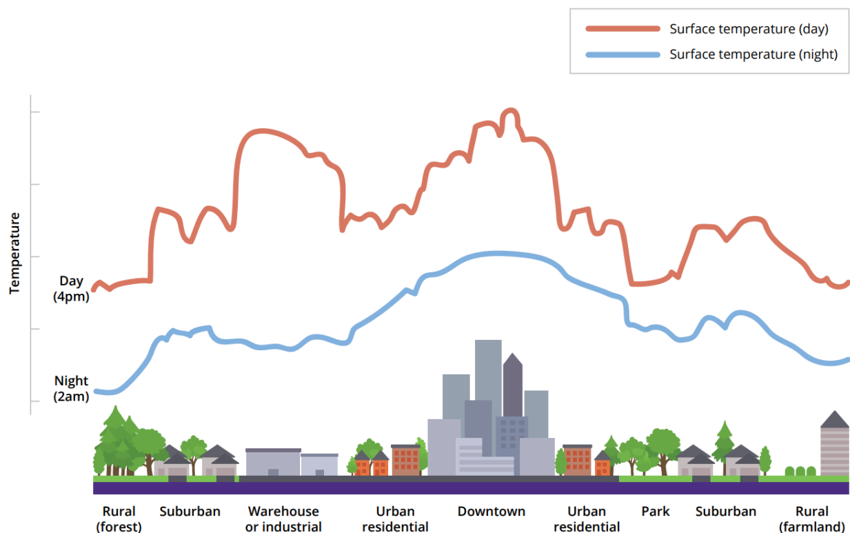
Figure 4.5-5 Day and night surface temperatures in a hypothetical urban heat island event.
