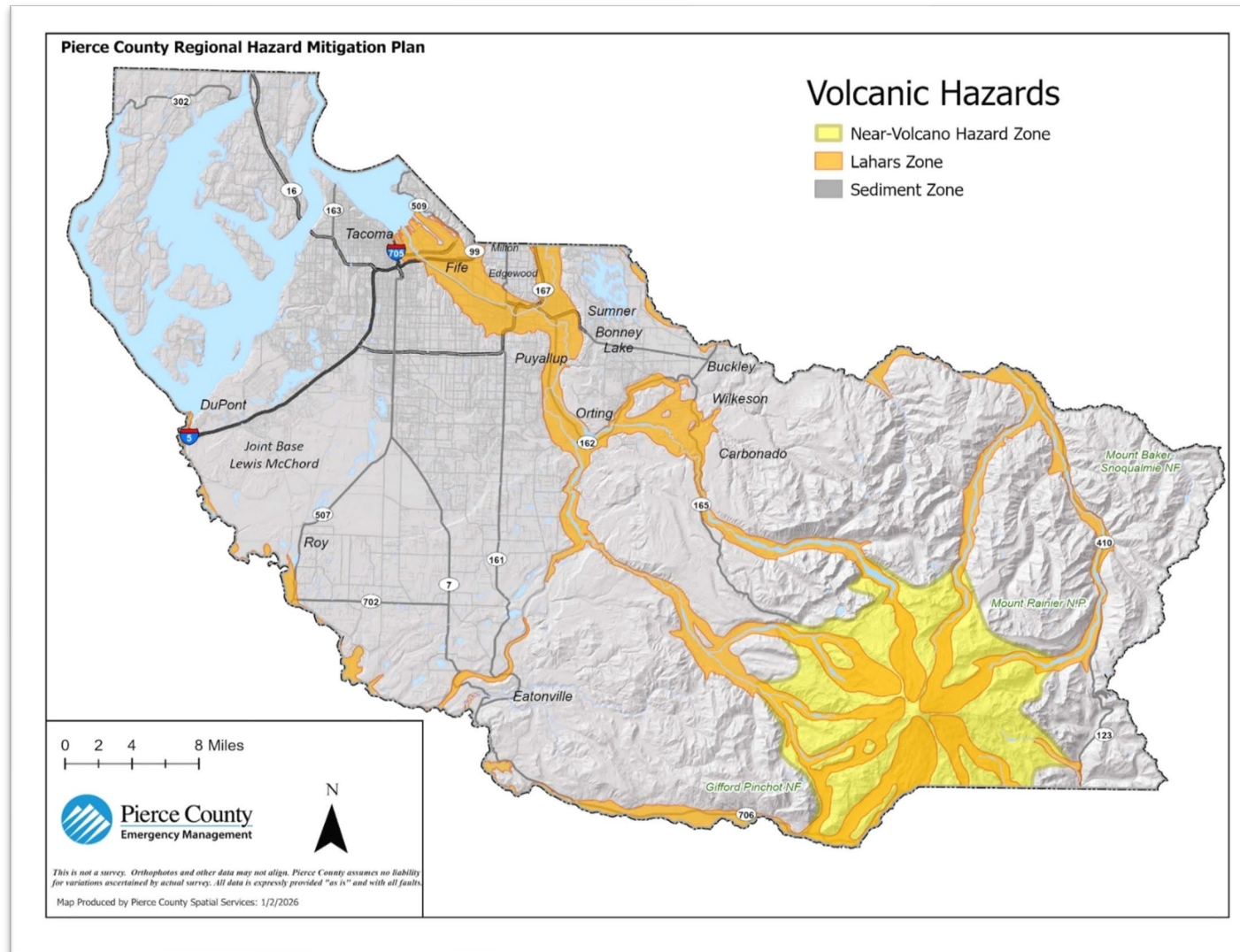
Map 4.7-2 Volcano and Lahar Hazards
