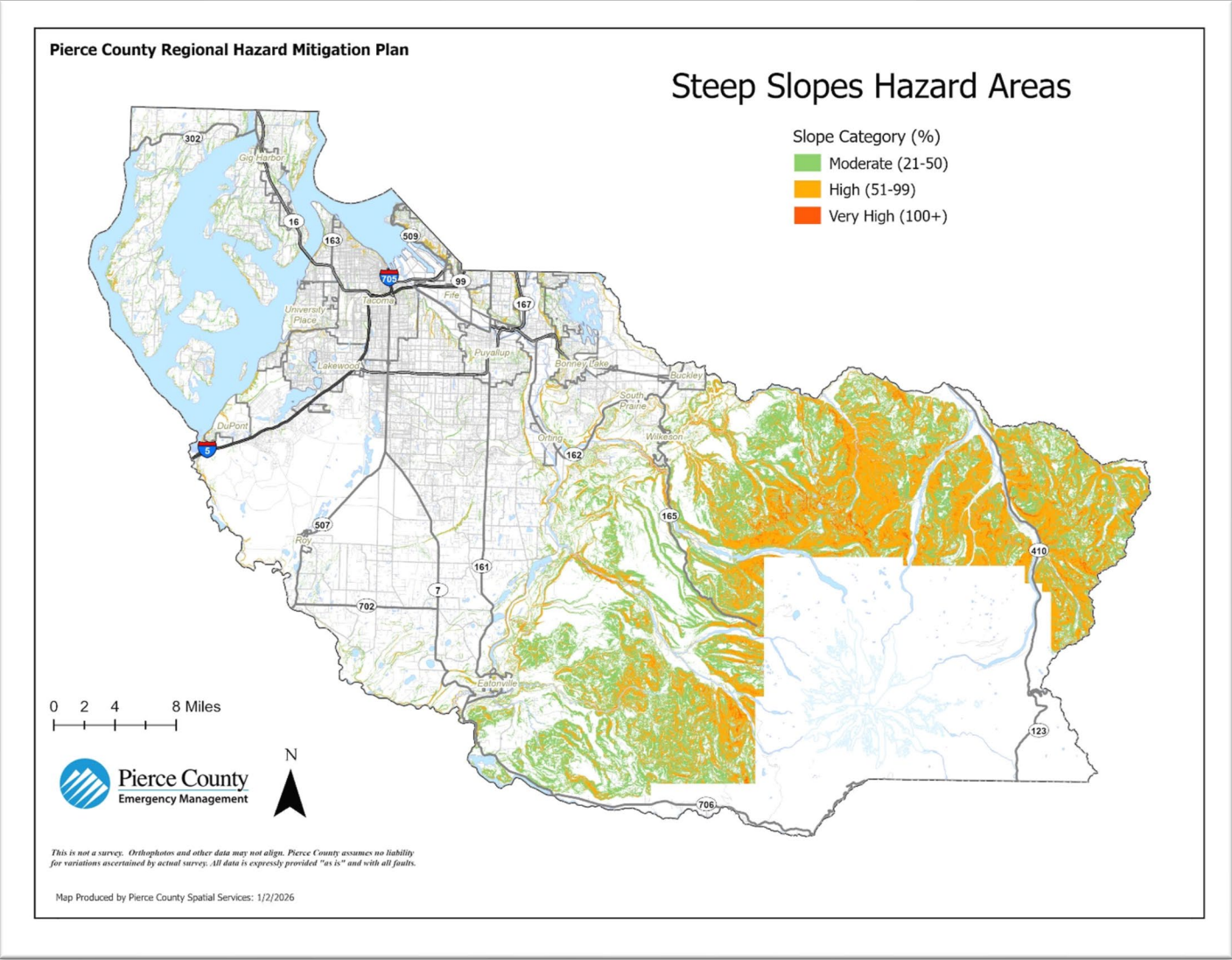
Map 4.4-3 Pierce County Steep Slopes Hazard Areas
