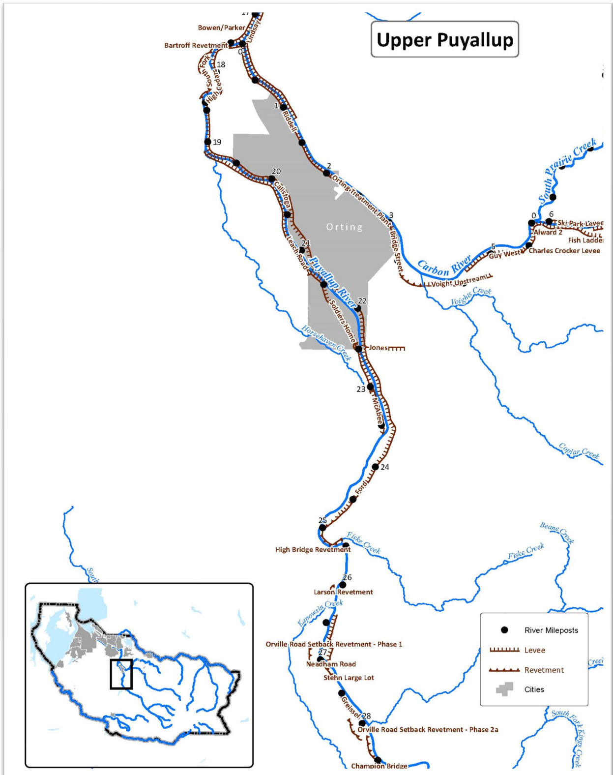
Map 4.3-4 Upper Puyallup River
