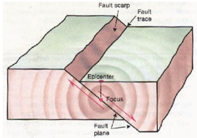
Figure 4.2-1 Diagram of an earthquake occurring at depth on a fault
