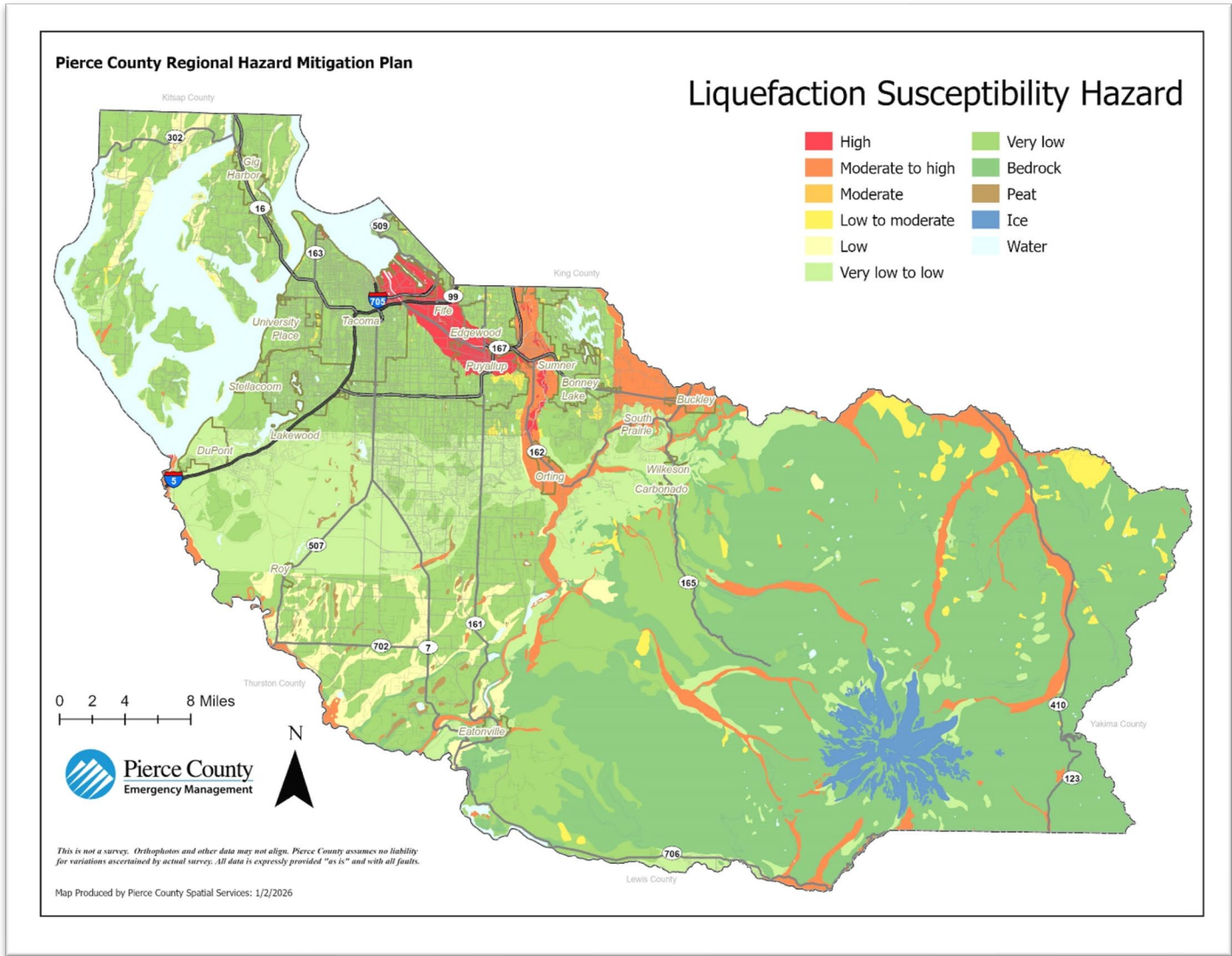
Map 4.2-1 Pierce County Earthquake Liquefaction Risk
