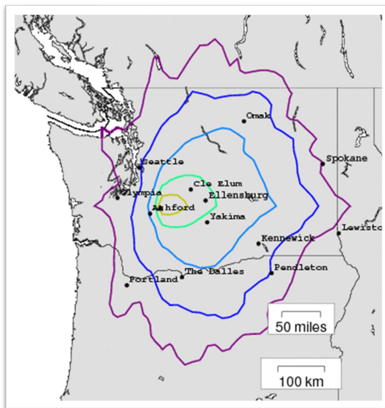
Map 4.7-3 Probability of Measurable Ashfall in Tacoma from Rainier
