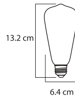
FOCO LED RETRO S14 1W E26 130V CLAVE S00773
