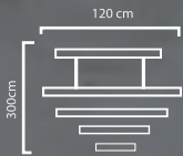
LUMINARIO TECHO LT LED SATIN CLAVE S00979 16W S00981 24W
