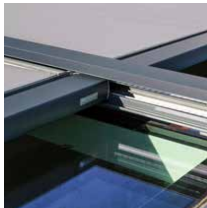
The hi-tensile, tear resistant dyneema cables are contained within the side guides
