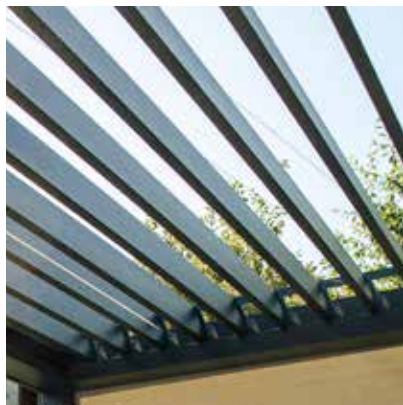
Wide 210mm double walled aluminium roof louvers rotate 150° for complete control over the sun
