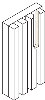
Presamaniglia fresata su anta Strike / Milled handle on Strike door
