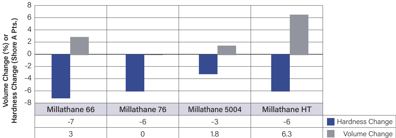
Immersion: IRM 903 Oil Immersion Test (70 hr/100°C) Black Reinforced, Peroxide Cured Polyester Millathane® Grades
