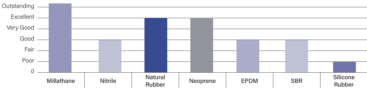
Abrasion Resistance (Relative)
