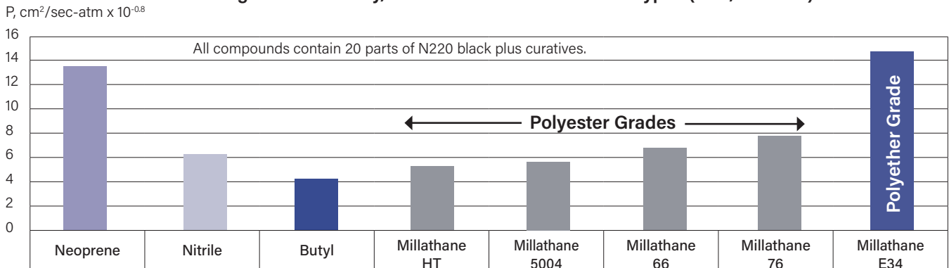
Nitrogen Permeability, Millathane vs. Other Rubber Types (80C, 345 kPa)
