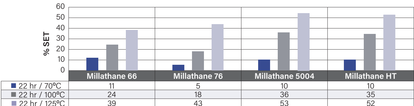
Compression Set Peroxide Cured Polyester Grade Millathane, Black Reinforced Compounds (ASTM D395 Method B)
