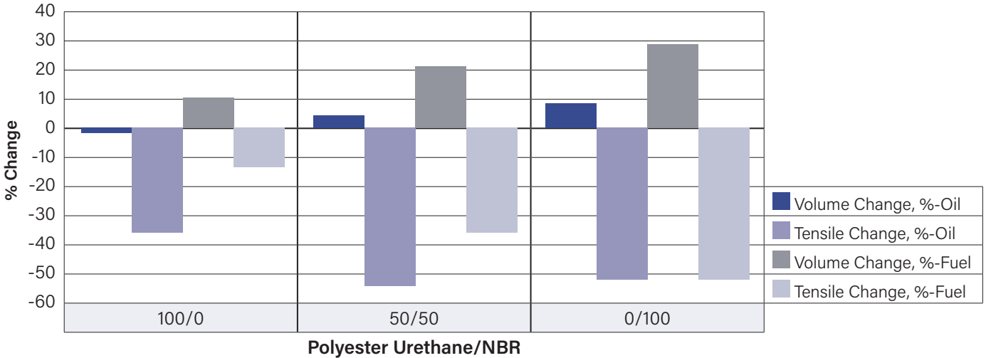
Immersion: IRM 903 Oil (70 hr/100°C) and Fuel B (7 d/23°C) Polyester Urethane vs. Medium ACN NBR (and 50/50 Blend)
