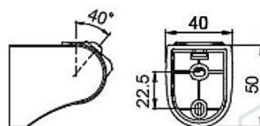
Bracket
