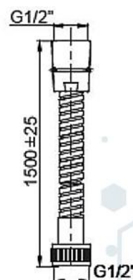
Hose
