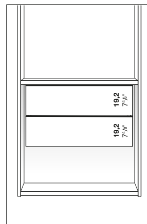
Suspended drawer chest 2 drawers Cassettiera sospesa 2 cassetti
