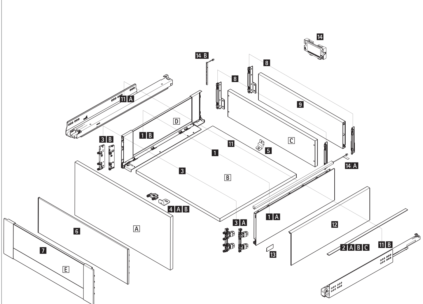
Exploded diagram
