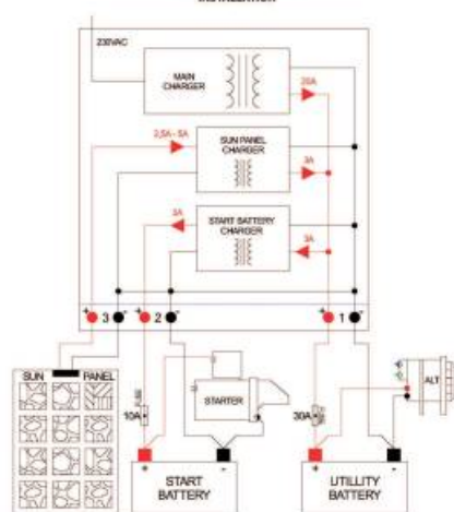
Dual output 12V/20A and 12V/3A and input from sun panel CCC12201203S03 INSTALLATION
