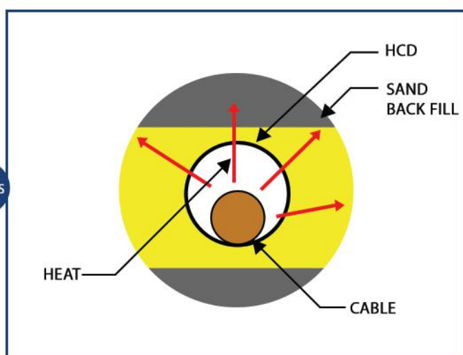
FIGURE 3. HDPE COIL DUCT WITH SAND BACKFILL HEAT IS NOT RETAINED INSIDE THE DUCT, ALLOWING FASTER HEAT TRANSFER TO THE SURROUNDING MATERIAL.
