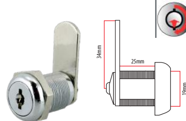
Fixings: Nut & Clip
