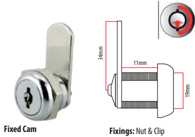
Fixings: Nut & Clip
