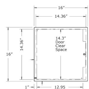
M3 Enclosure
