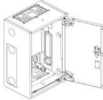
PRO IP40 S13 (b=300, h=500, d=210mm)
