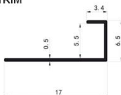
EXTERNAL TRIM
