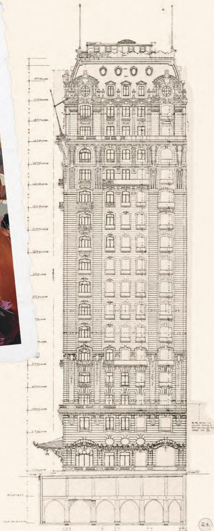
FIFTH AVE. ELEVATION SCALE 1/4" = 1'
