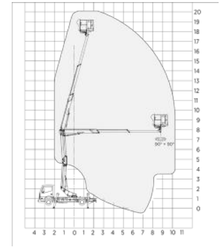
OIL&STEEL SNAKE 2010 PLUS
