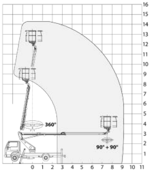
OIL&STEEL SCORPION 1490
