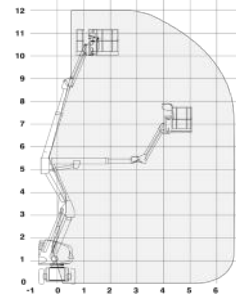
HAULOTTE HA12IP
