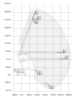
GENIE Z-80/60
