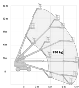
JLG 460SJ
