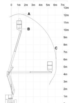
NIFTYLIFT HR 12 N
