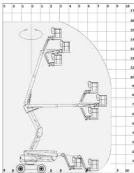
MANITOU 160ATJ
