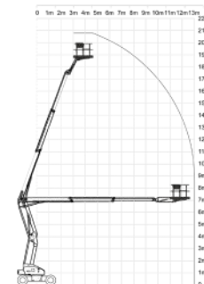
NIFTYLIFT HR21D
