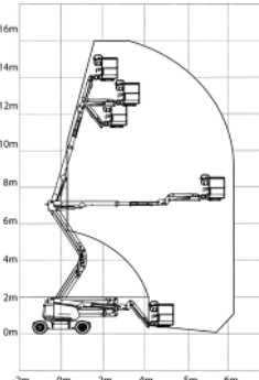
LGMG AR16J
