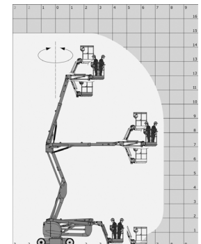
MANITOU 150AETJC
