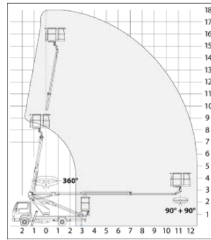
OIL&STEEL SCORPION 1812
