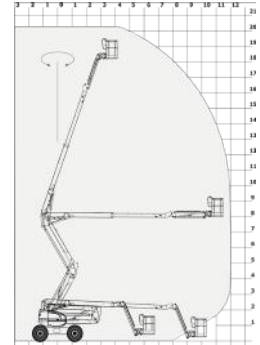
MANITOU 200ATJ
