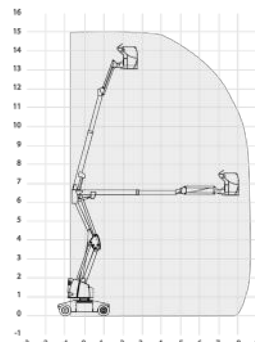
HAULOTTE HA15IP
