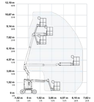
GENIE Z-30/20N
