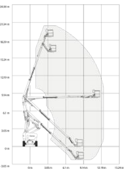
GENIE Z-62/40
