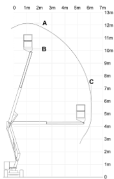
NIFTYLIFT HR12N
