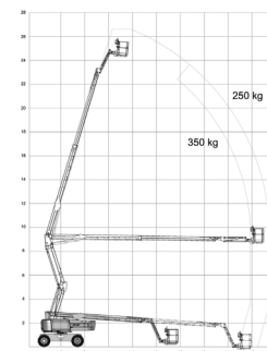
HAULOTTE HA26RTJ PRO
