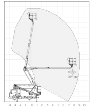
OIL&STEEL SNAKE 189
