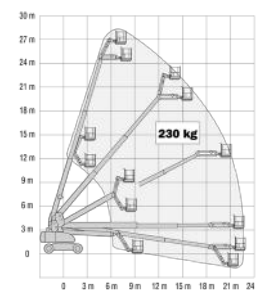
JLG 860SJ
