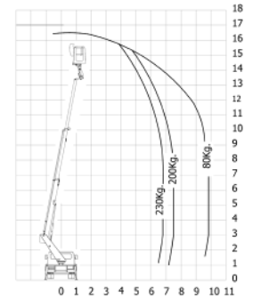
MOVEX TLR 16
