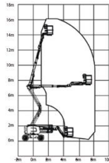
LGMG AR14J
