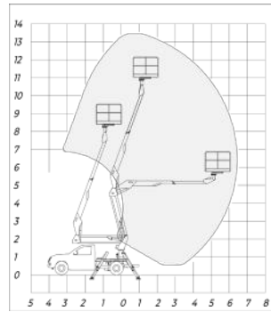
SOGAGE 14A (Pick-up)
