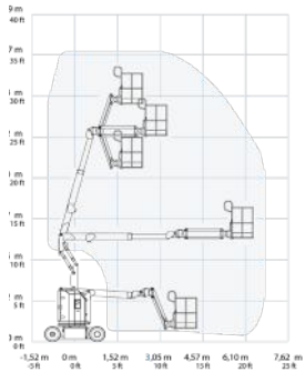
GENIE Z-30/20NRJ
