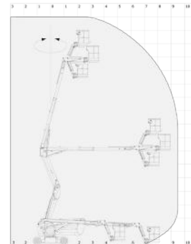
MANITOU 170AETJL
