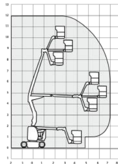
MANITOU 120AETJC
