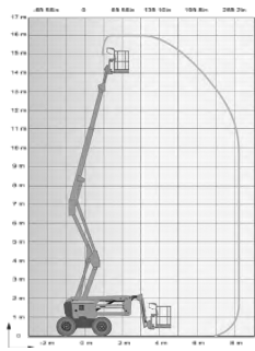
HAULOTTE HA16RTJ
