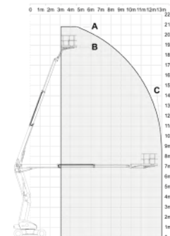
NIFTYLIFT HR21 HYBRID MK1B
