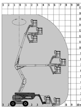
MANITOU 180ATJ
