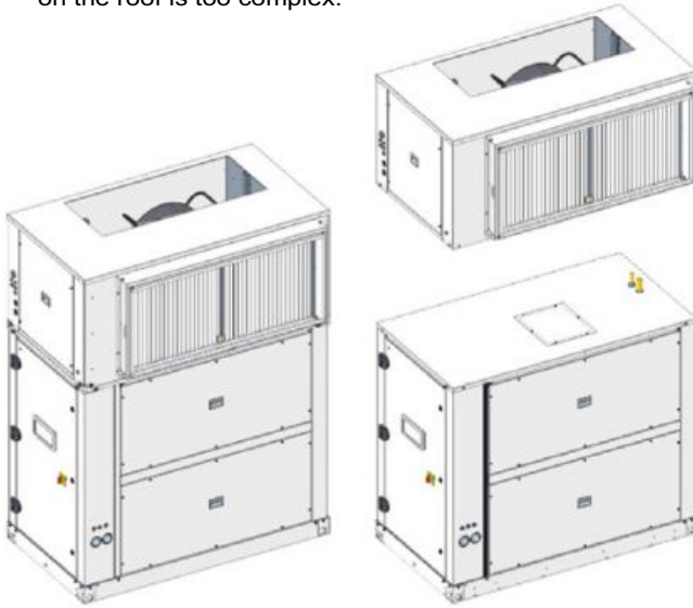
Package version
