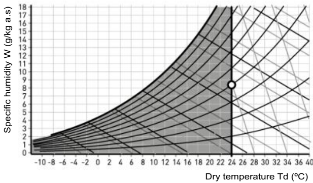
Thermal free-cooling
