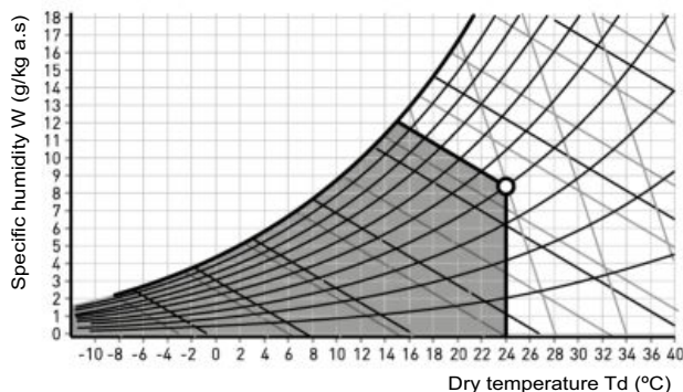
Thermoenthalpic free-cooling
