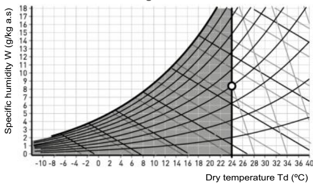
Thermal free-cooling
