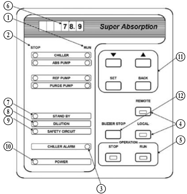
Figure 11 - Display panel
