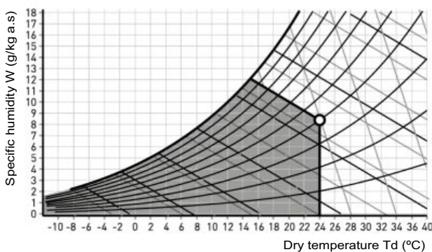
Thermoenthalpic free-cooling
