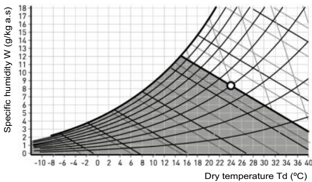
Enthalpic free-cooling
