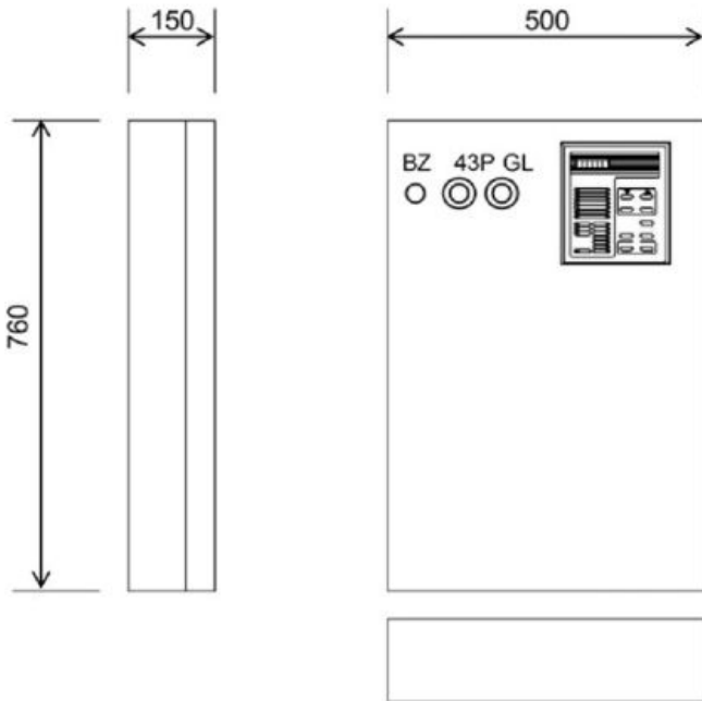
Figure 10 - Control panel
