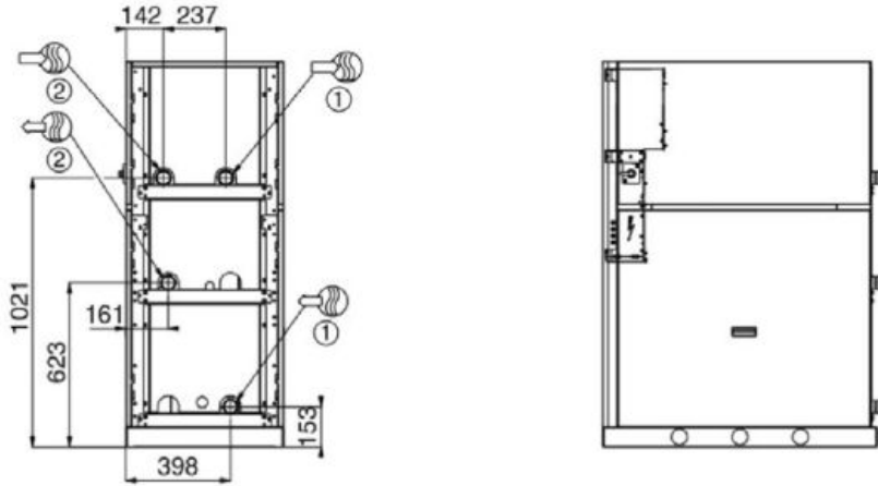
30WG 020-045 - unit with evaporator/condenser hydraulic modules (options 116 + 270)
