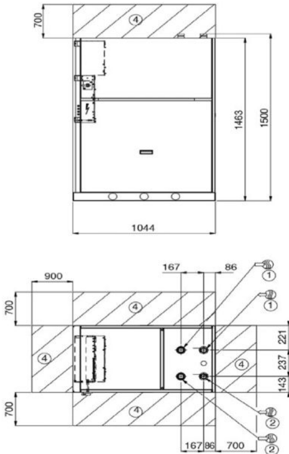
30WG 020-045 - unit with hydraulic module and top connections (options 116 + 274 or 270 + 274 or 116 + 270 + 274)
