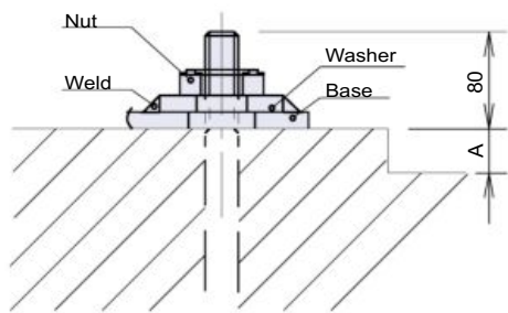
Figure 4 - Details of weld
