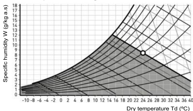
Enthalpic free-cooling
