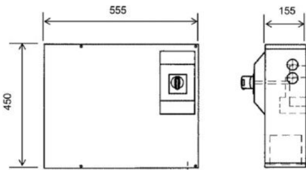
Figure 12 - Power panel
