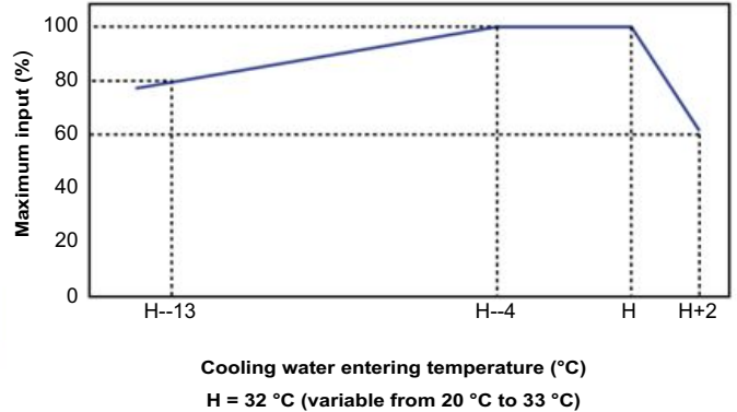
Graph 6 - Safe operating zone chart
