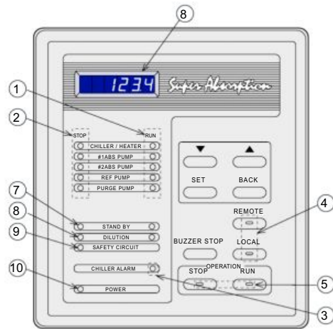
Figure 2 - Indication lights
