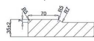
Tray Profile
