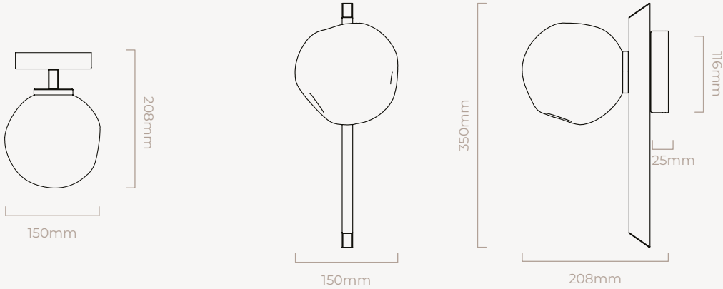
DALI B included - The light will feature a deeper wall rose. For use when there is no space in the existing wall cavity
