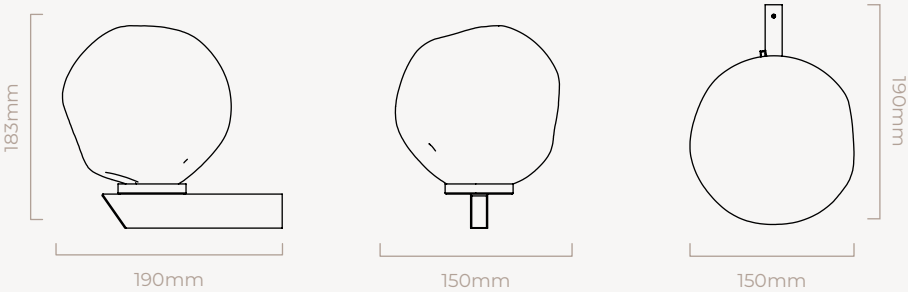
DALI A included - For lights that do not require aesthetic alterations. Dali can be fitted inside the wall cavity
