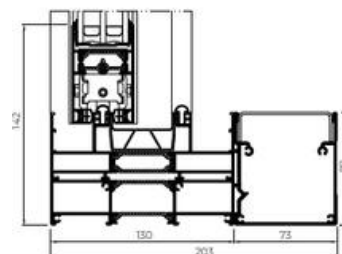
Embedded Frame With Groove
