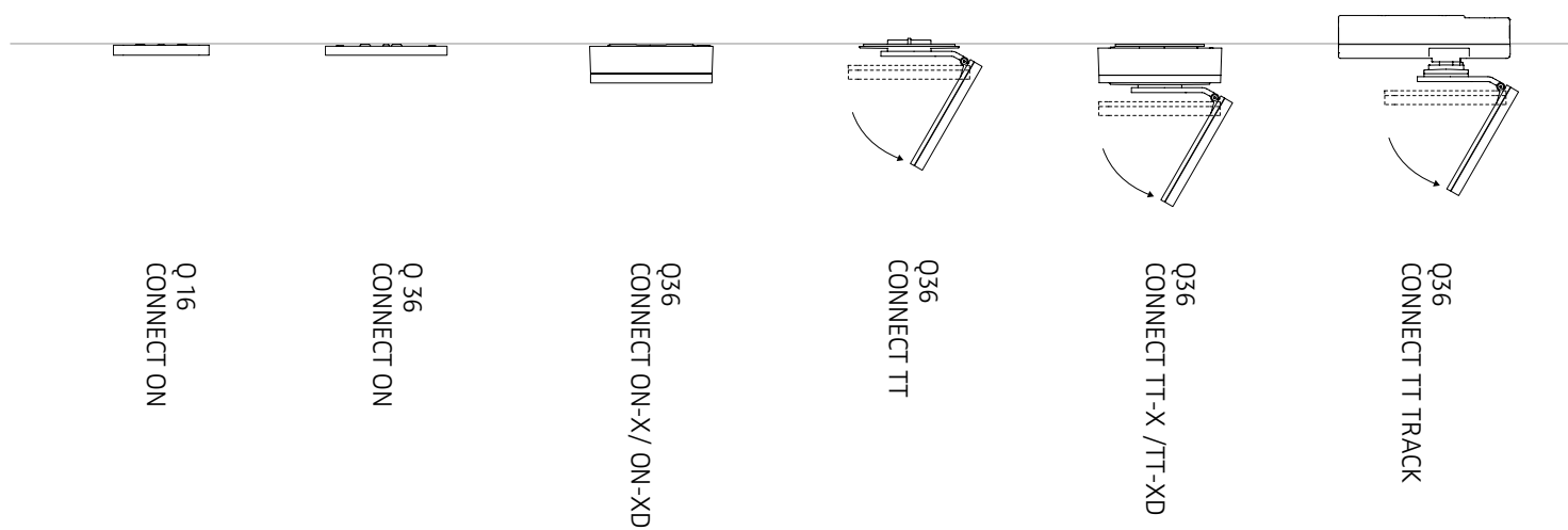
MODUL Q CONNECT PRODUKTFAMILIE MODUL Q CONNECT PRODUCT FAMILY
