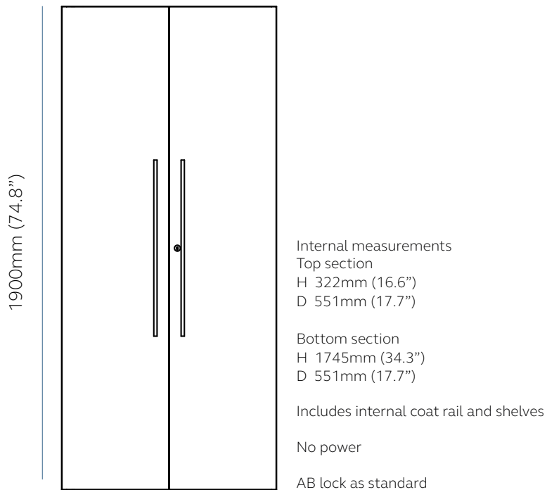
Coat cupboard
