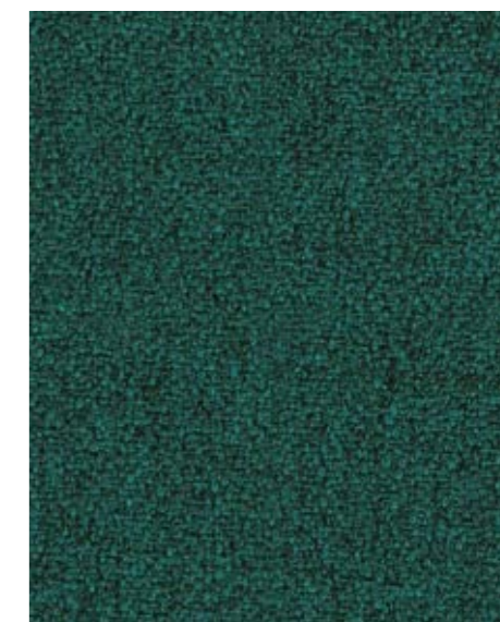
Ratio AK001
