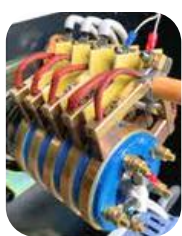
Anillo colector
