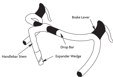
Racing Handlebar Assembly
