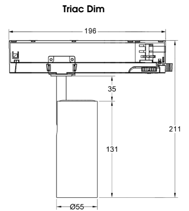
Dimmer on Adapter
