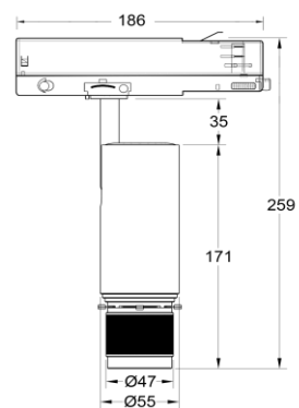
Dimmer on Adapter
