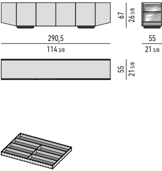
CONTENITORE ORIZZONTALE DINING CM 290,5X55 H67 DINING HORIZONTAL SIDEBOARD CM 290,5X55 H67
