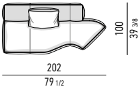
SOFA ELEMENTO CENTRALE INCLINATO CM 202X100 - SX/DX SOFA INCLINED CENTRAL ELEMENT CM 202X100 - SX/DX
