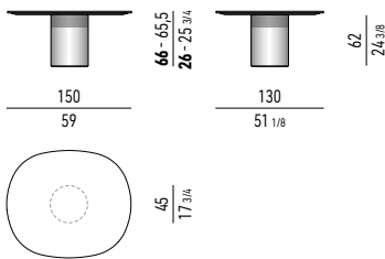
PIANO IN LEGNO | WOOD TOP: CM H 65,5 PIANO IN MARMO | MARBLE TOP: CM H 66
