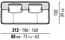
SOFA ELEMENTO CENTRALE CM 212X100 - 186X100 - 160X100 SOFA CENTRAL ELEMENT CM 212X100 - 186X100 - 160X100
