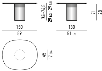
PIANO IN LEGNO | WOOD TOP: CM H 74,5 PIANO IN MARMO | MARBLE TOP: CM H 75
