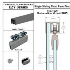
EZY1HSDP (Heavy Duty) Single Door + Fixed Panel Kit
