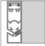
Montante anteriore fianco Skeltro con luce LED /Skeletro front pillar of the side with LED light
