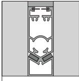
Montante anteriore divisione Skeltro con luce LED /Skeletro front pillar of the partition with LED light
