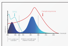
O-light plus spectral curve & resin spectral absorptivity
