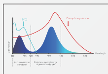
O-light plus spectral curve & resin spectral absorptivity
