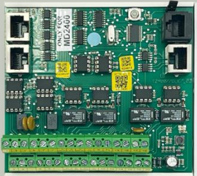
MD2400 – redundantie Token-ring & I/O bus Ref. 243264
