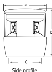
Side profile
