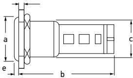
Buzzer
