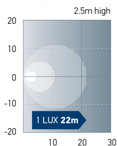
FMS1200 Light Distribution
