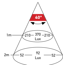
EuroLED 150
