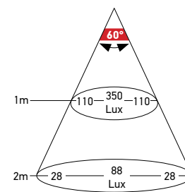
6500 K - 20 LED
