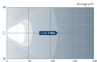
Extra Wide 011872521
