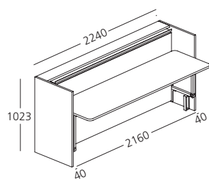
Cabrio In, fianchi laterali
